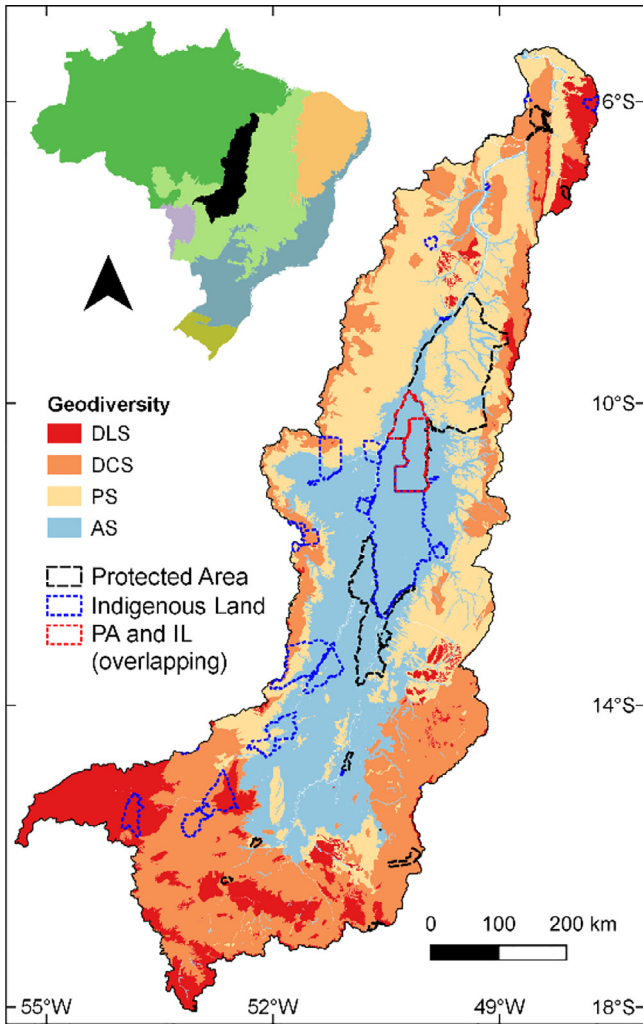
Fig. 2. Geodiversity map at 1:250,000 scale from CPRM, 2014 [6].
