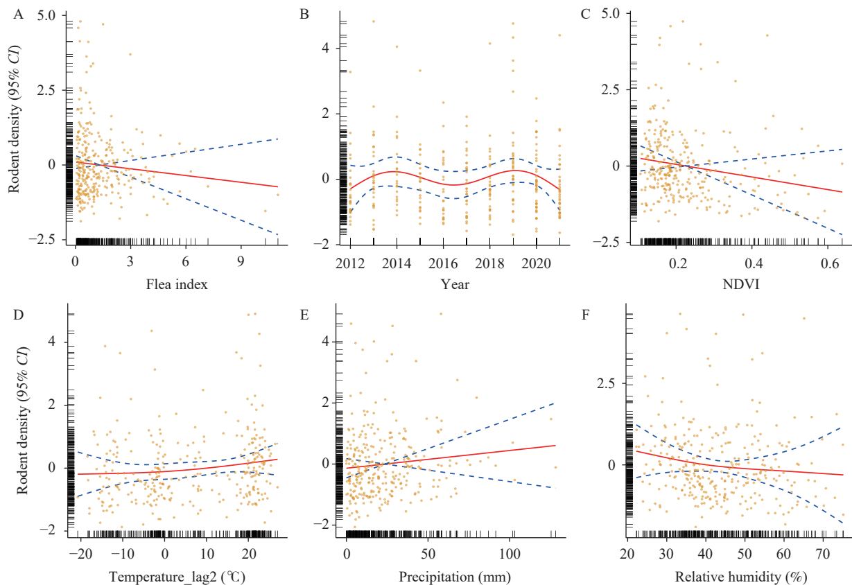
FIGURE 1. Analysis of factors influencing the density of Mongolian gerbils in Xilingol League from 2012 to 2021 using generalized additive modeling. (A) The correlation between flea index and rodent density; (B) The association between time trend (year) and rodent density; (C) The link between NDVI and rodent density; (D) The connection between monthly average temperature with a 2-month lag and rodent density; (E) The correlation between monthly cumulative precipitation and rodent density; (F) The relationship between monthly average relative humidity and rodent density. Abbreviation: NDVI=normalized difference vegetation index; CI=confidence interval.
