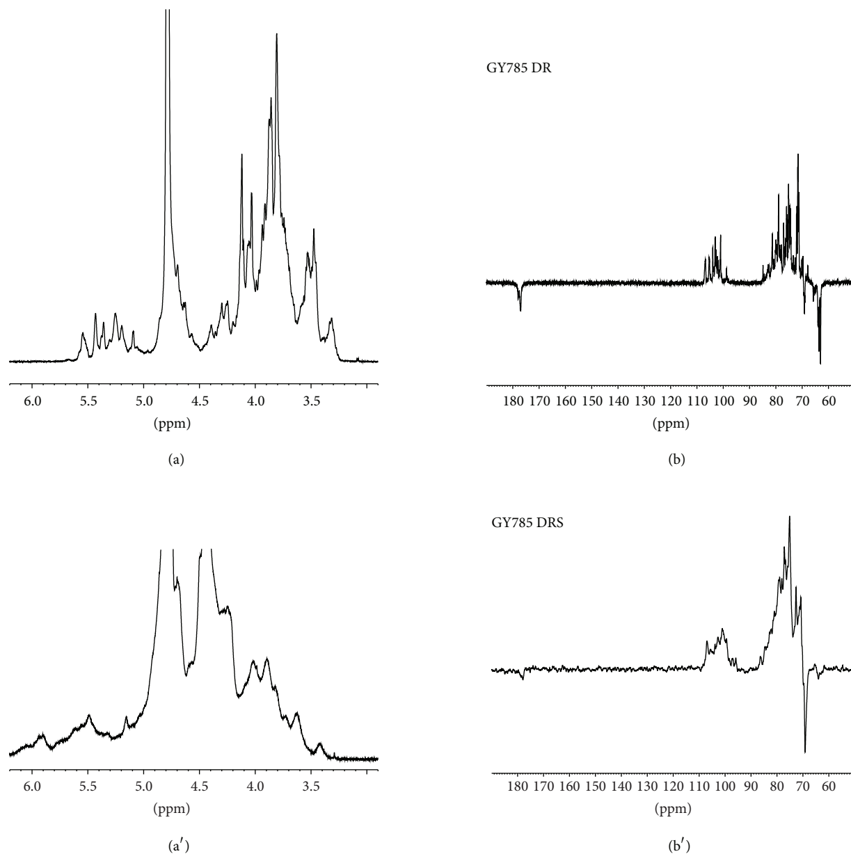
FIGURE 4: 1 H NMR spectra of GY785 DR (a) and GY785 DRS (a') and 13 C J-modulated NMR spectra of GY785 DR (b) and GY785 DRS (b').
