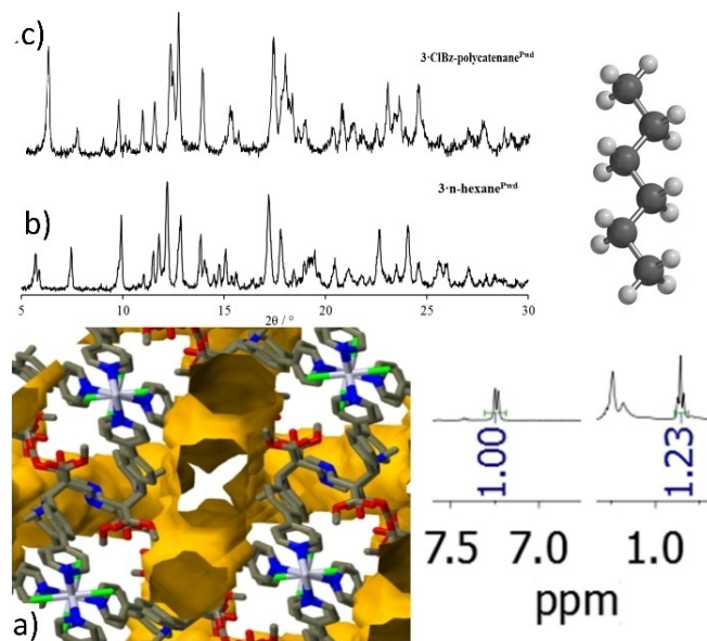
Figure 10. a) View of the void space (25%) potentially available by removal of ClBz molecules from the interconnected channel of 3·ClBz-polycatenane SC . b) P-XRD pattern of the CP obtained by exposure of 3·ClBz-polycatenane PwD (whose P-XRD pattern is shown in c) to n -hexane vapours. 1 H-NMR R value is 0.82.
