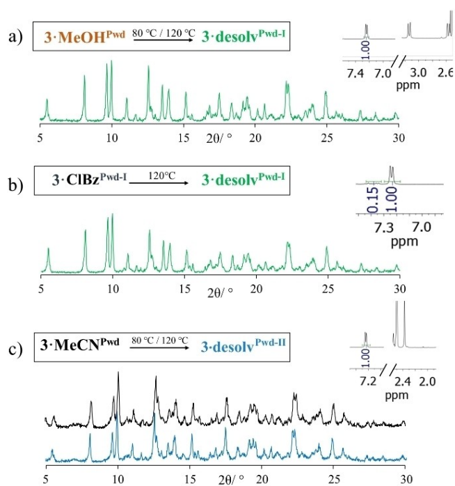
Figure 8. Summary of the thermal treatment performed on CPs and their outcome. Experimental P-XRD pattern of CP obtained from thermal treatment of a) 3 \cdot \text{MeOH}^{\text{Pwd}} at 80 °C or 120 °C; b) 3 \cdot \text{ClBz}^{\text{Pwd-I}} at 120 °C and c) 3 \cdot \text{MeCN}^{\text{Pwd}} at 80 or 120 °C. Portions of relevant corresponding ^1\text{H} NMR spectra are shown, indicating no solvent present (400 MHz, 302 K, \text{DMSO-}d_6 ).
