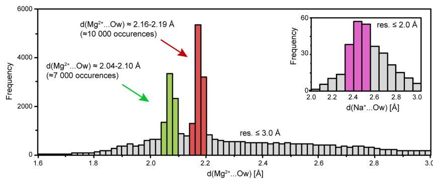
Figure 11. d(\text{Mg}^{2+} \dots \text{Ow}) histogram for nucleic acid crystal structures (PDB; May 2016; resolution \leq 3.0 \text{ \AA} ) that emphasize the systematic use of crystallographic restraints around 2.07 and 2.18 \text{\AA} . The d(\text{Na}^+ \dots \text{Ow}) histogram peaks around 2.4 \text{\AA} and no peaks associated with crystallographic restraints are apparent (see insert; resolution \leq 2.0 \text{ \AA} ). Supplementary Figure S9 displays d(\text{Mn}^{2+}/\text{Na}^+ \dots \text{Ow}) histograms where peaks due to the use of restraints are also absent (resolution \leq 3.0 \text{ \AA} ).
