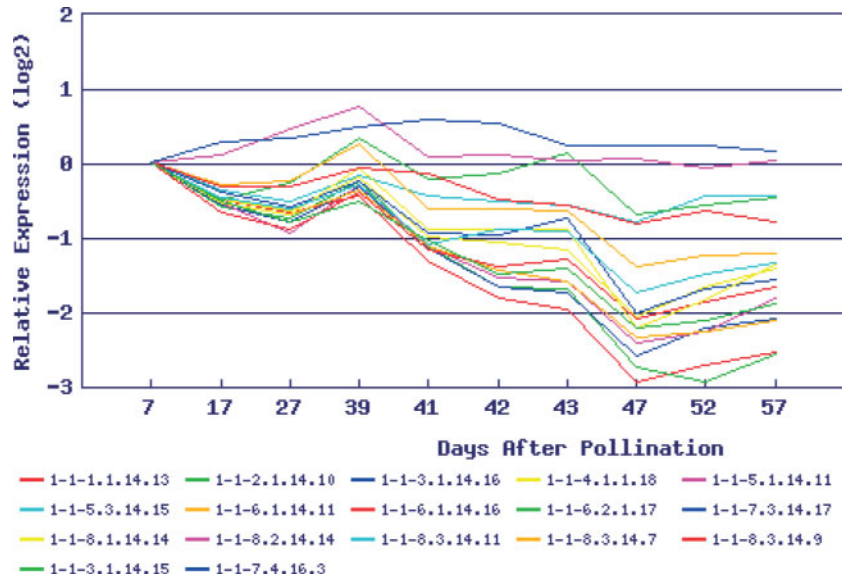
Figure 2. Pseudo-replica Expression. Expression profiles of pseudo-replicates from unigene SGN-U212746, a putative peptidyl-prolyl cis-trans isomerase, during normal tomato fruit development and ripening.
