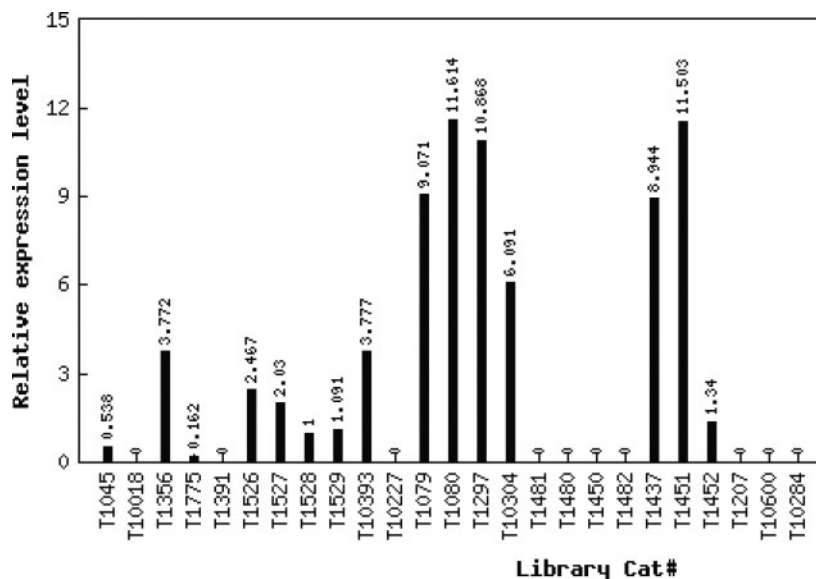
Figure 4. Visualization of digital expression in TED. Normalized digital expression profile of tomato TC115712, a putative plastidic aldolase.
