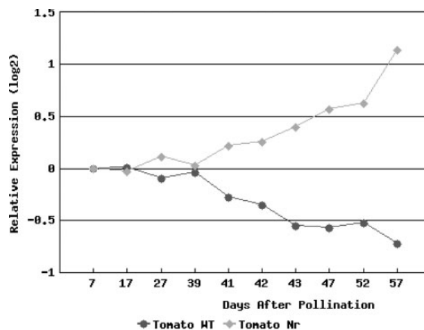
Figure 1. Cross Genotype Comparison Tool. Comparison of expression profiles of 1-1-3.4.10.21, a Pto-like serine/threonine kinase, during normal tomato and Nr mutant fruit development. The Pearson correlation coefficient ( r ) of the two profiles is -0.9254 .
