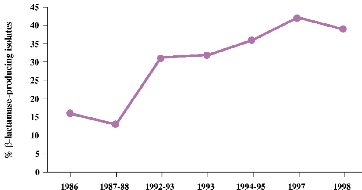
Fig 8. Prevalence of \beta -lactamase production by H influenzae in the United States from 1986 to 1998.
