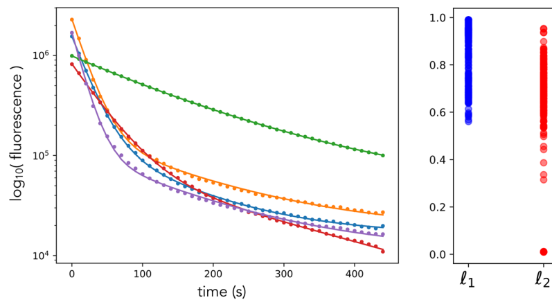
Figure 2. Photobleaching in vivo is not described by a homogeneous, single exponential decay. Left: The logarithm of the fluorescence of 5 cells of budding yeast expressing Pgc1-GFP and undergoing photobleaching do not all fall on a straight line as a function of time (c.f. Fig. 1). The data are shown as dots and the fits for double exponential decay as lines, which is modelled for fluorescence at time point i as f_i = a_0 + a_1 \ell_1^i + a_2 \ell_2^i with constants a and \ell_1 = e^{-\lambda_1 \Delta t} and \ell_2 = e^{-\lambda_2 \Delta t} for time scales \lambda and time \Delta t between measurements (here 10 s). All data have been corrected for autofluorescence using wild-type cells that do not express GFP. Right: bleaching is heterogeneous across the population of cells. There is substantial cell-to-cell variation in the best-fit values for \ell_1 and \ell_2 .
