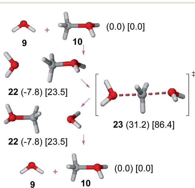
Fig. 4 S_N2 mechanism. Relative Gibbs free energies ( \text{kJ mol}^{-1} ) in gas phase (in parenthesis) and solution (in square brackets) of involved structures are shown.
