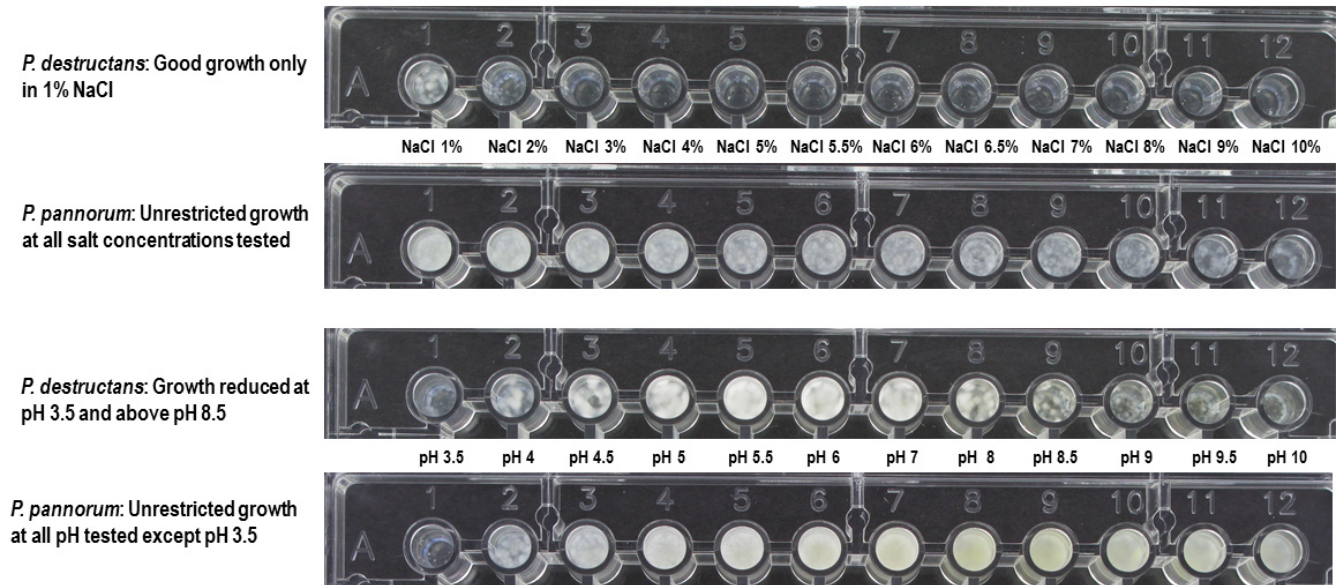
Figure 5. Growth of Pseudogymnoascus destructans and Pseudogymnoascus pannorum under high salt and pH extremes.
