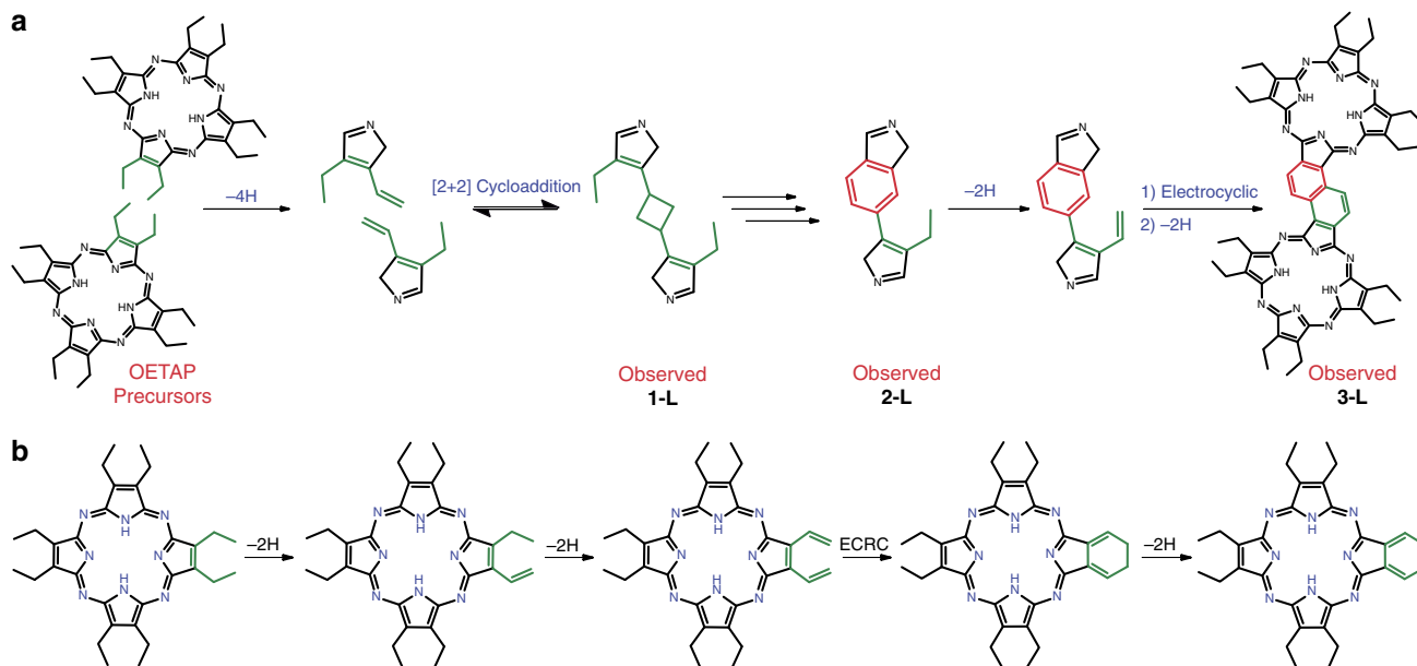
Figure 5 | Proposed reaction mechanisms describing the surface-assisted formation of phthalocyanine polymers and monomers on Au(111).
