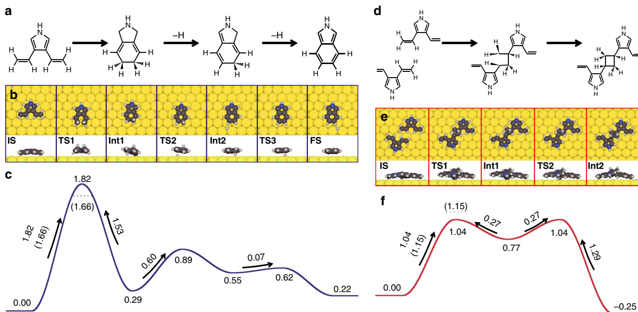
Figure 6 | Reaction pathway considerations for a model pyrrole molecule on Au(111). (a–c) Monomer cyclization. (d–f) Initial steps of the dimerization process. For both reactions, it is assumed that the ethyl legs have been transformed into ethenyl groups through dehydrogenation reactions, the details of which are shown in the Supplementary Information. (a,d) Chemical stick models and (b,e) top and side view ball models for reactants (IS), transition states (TS), reaction intermediates (Int) and the monomer reaction final state (FS). (c,f) Energy profiles for the monomer cyclization and initial steps of the dimerization process, respectively. Free energy barriers are shown in parentheses and indicated by the dotted lines for TS1 of each reaction, calculated by including vibrational enthalpy and entropy at 275 °C. Energies are given in units of eV.
