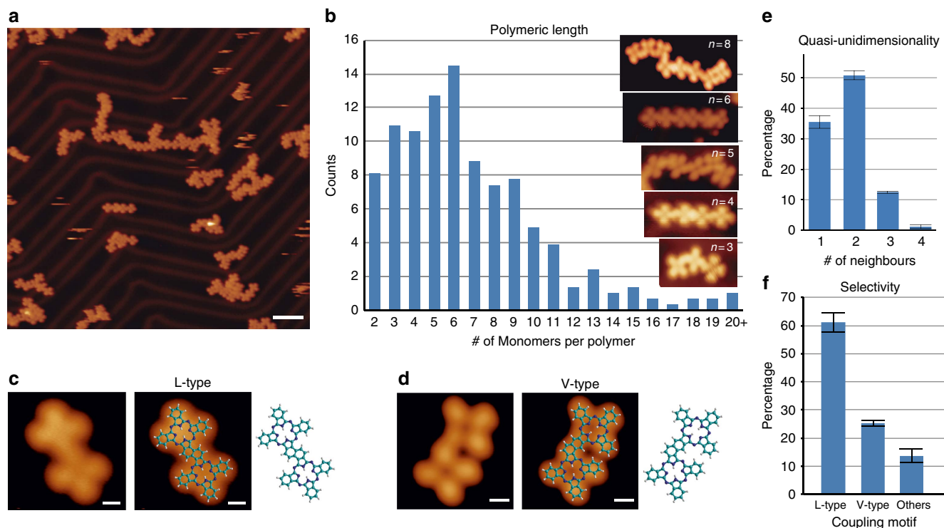
Figure 2 | Surface-confined synthesis of phthalocyanine tapes. The deposition of 0.3 ML of OETAP species (precursors) on Au(111) held at room temperature and subsequent gently annealing at 275 °C affords the formation of phthalocyanine polymers. (a) Long-range STM image displaying the formation of quasi-unidimensional polymers mainly confined to the fcc regions. (b) High-resolution STM images of polymers of distinct size (3, 4, 5, 6 and 8) and histogram of the polymeric length. (c,d) High-resolution STM image and models of the majority of products between coupled monomers ( c , L-type and d , V-type). (e) Histogram of the number of neighbours per monomer, highlighting the quasi-unidimensional feature of the assemblies. (f) Histogram of different types of coupling motifs exhibiting selectivity towards L-type-binding motif. Errors bars in e,f are the standard deviation of the mean. Tunnelling parameters: a , V_b = -1.5 V; b , V_b = -0.5 V for n=3 , V_b = -1.5 V for n=4 , V_b = -1 V for n=5 , V_b = -1 V for n=6 , V_b = -1 V for n=6 , V_b = -1.2 V for n=8 ; c , V_b = -1.5 V and d , V_b = -0.7 V. Scale bars, a , 5 nm; c,d , 0.5 nm.
