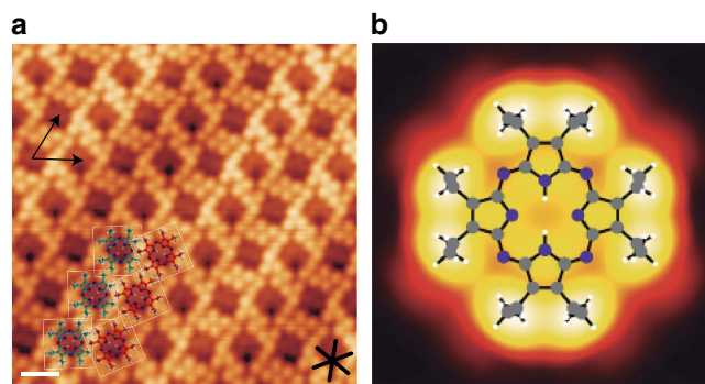
Figure 1 | Self-assembly of OETAP on Au(111) after deposition at room temperature. (a) High-resolution STM images revealing submolecular features. Black arrows depict the lattice vectors of the rhombic unit cell. Black star shows the close-packed directions of the surface. Superimposed coloured atomistic models address the two distinctly oriented molecular species (green and red, respectively). Tunnelling parameters: V_b = 0.5 V, I = 0.1 nA. Scale bar, 1 nm. (b) STM simulated image of an individual OETAP on Au(111) at 0.5 V, with a superimposed ball-and-stick model of the molecular species. Hydrogen, carbon and nitrogen atoms are depicted in white, grey and violet, respectively.
