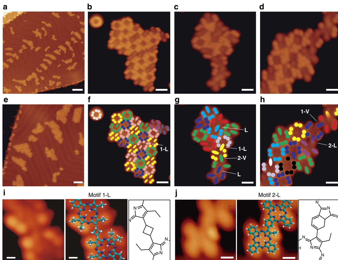
Figure 4 | Surface-assisted formation of phthalocyanine derivatives after deposition of OETAP precursors on Au(111). (a,e) Large-scale STM images showing the formation of patches of initially reacted molecules coexisting with unreacted species. (b–d) High-resolution STM images and (f–h) corresponding schematic colouring of the initial steps of reactions giving motifs 1-L , 1-V , 2-L , 2-V and L . (i,j) Zoom-in of motif 1-L and 2-L , and superimposed modelling, together with chemical drawing insets. Coloured filled dots represent ethyl moieties, bi-coloured ellipses show covalent connections between adjacent species, and mono-coloured ellipses represent full electrocyclic ring closures. Tunnelling parameters: a , V_b = -0.8 V; b , V_b = -0.7 V; c , V_b = -0.7 V; d , V_b = -0.8 V; e , V_b = -1.2 V; i , V_b = 0.5 V and j , V_b = -1.5 V. Scale bars, a , 10 nm; b , 1.5 nm; c , 1.0 nm; d , 1.0 nm; e , 5 nm; f , 1.5 nm; g , 1.0 nm; h , 1.0 nm; i , 0.3 nm and j , 0.5 nm.
