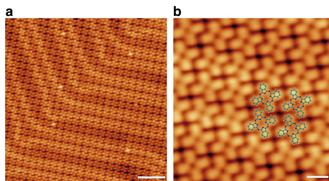
Figure 3 | Surface-assisted synthesis and self-assembly of phthalocyanines. The deposition of OETAP species on Au(111) held at 300 °C affords the on-surface chemical transformation of precursors into phthalocyanine species. (a) Long-range STM image, revealing the close-packed supramolecular assembly and highlighting the presence of the herringbone reconstruction of Au(111). (b) High-resolution STM image and superimposed modelling of the molecular constituents, which matches the reported assembly of 2H-Pc on Au(111). a,b , V_b = -1 V. Scale bars: a , 5 nm; b , 1 nm.
