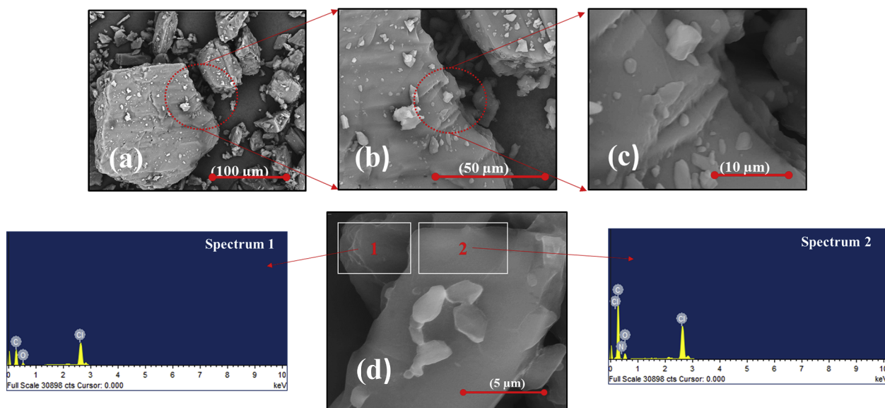
Fig. 6. Characterisation of PPN surface using SEM/EDX. SEM images at different magnifications \times 500 (a), \times 1500 (b), \times 5000 (c) and \times 10,000 (d); atomic distribution profile at two different sample locations (Spectrum 1 and 2).
