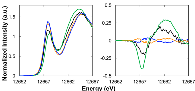
Figure 6. Experimental Se HERFD XAS (left) and corresponding difference spectra (right) of Av1Se 10 (blue), Av1Se hi (orange), Av1Se reac (black), and Av1SeCO (green). The difference spectra are taken relative to the average of Av1Se 10 and Av1Se hi .
