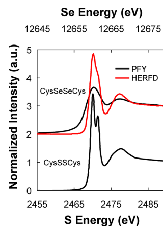
Figure 2. Comparison of S and Se K-edge partial fluorescence yield (PFY) XAS spectra of cystine (bottom) and selenocystine (top, black) with high energy resolution fluorescence detected (HERFD) Se K-edge XAS spectra of selenocystine (top, red). HERFD data are from the present study. PFY data are adapted from ref 54 with permission from the Society of Biological Inorganic Chemistry (1999).
