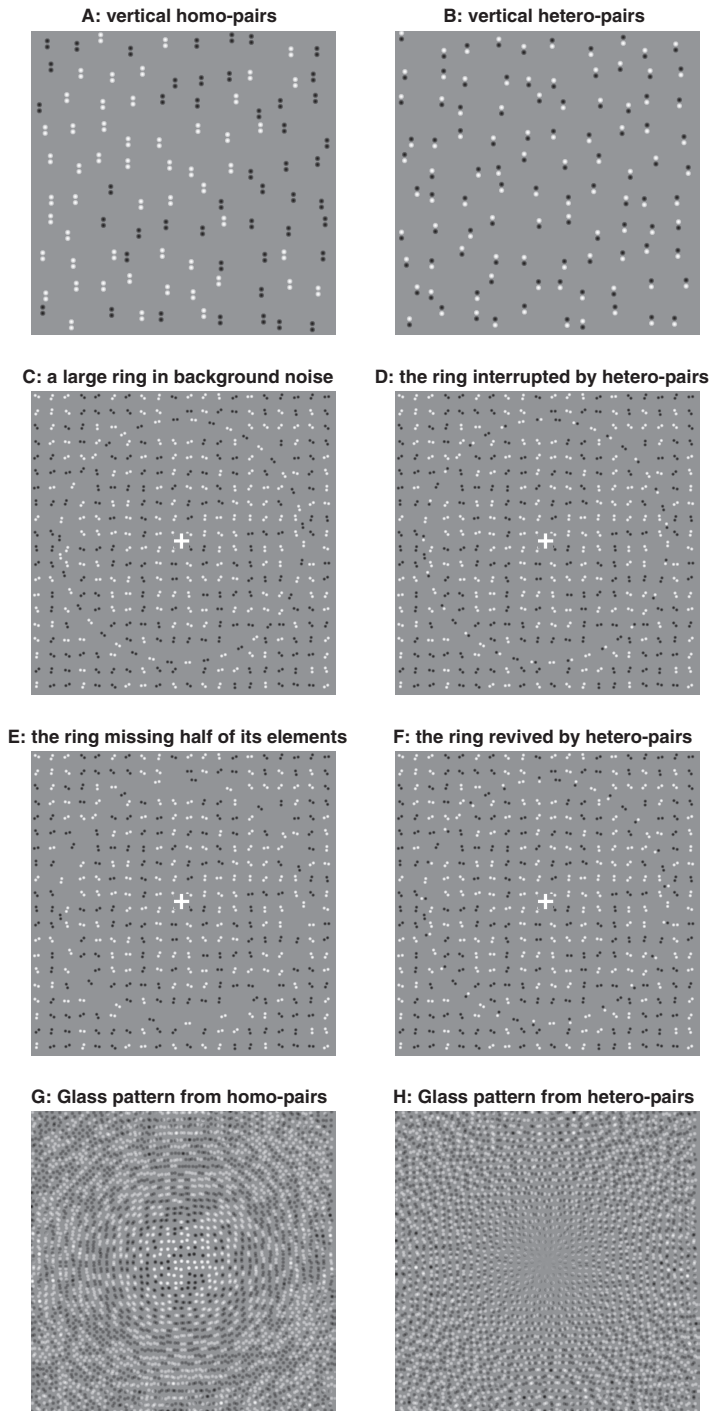
Figure 1. Vertical homo- (A) or hetero-pairs (B). Viewed peripherally, the pairs in (B) appear horizontal. C–F: Fixate the central cross, the large ring (in background noise) is more noticeable in (C) and (F) than (D) and (E). Only the elements of the rings differ. (G) and (H): Glass patterns by superposing a field of black and white dots and its slightly (by 2^\circ ) rotated (and contrast-inverted for H) version.
