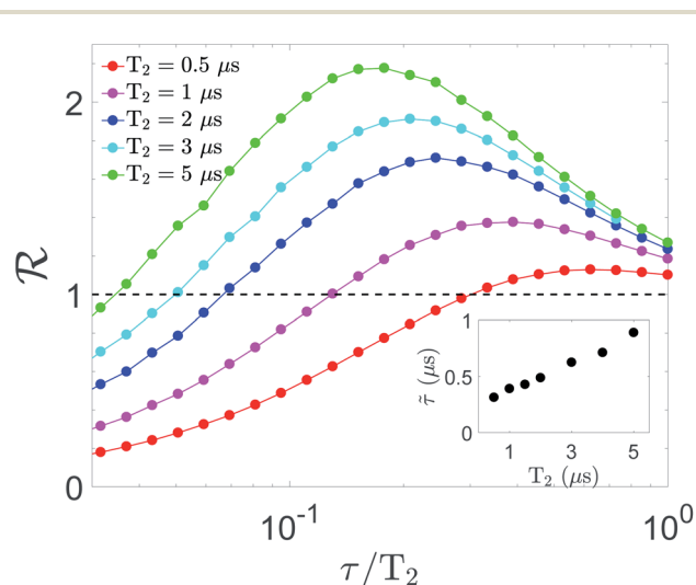
Fig. 4 Gain \mathcal{R} after correction as a function of memory time \tau/T_2 , for different values of T_2 , corresponding to different colours. \mathcal{R} is given by the ratio between error on an isolated qubit \mathcal{E}_U = 2|\alpha|^2|\beta|^2(1 - e^{-\tau/T_2}) and after implementation of the TQC, \mathcal{E}_C . This shows a maximum at \tau = \tilde{\tau} , reported in the inset as a function of T_2 . We work in a static field B_z = 1 T, use magnetic pulses of peak amplitude 50 G and choose \alpha = -i\beta = 1/\sqrt{2} .
