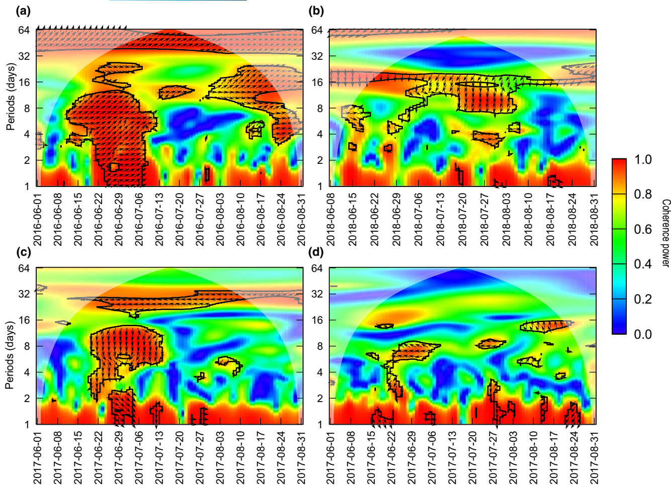
FIGURE 2 Wavelet coherence analysis between dissolved organic carbon concentrations and discharge (a), gross primary production (b), net ecosystem production (c), ecosystem respiration (d) in summer 2016, 2018, 2017 and 2017, respectively. The colours of power values range from blue (low values) to green (intermediate) to red (high values). The red parts inside the black border indicate significantly temporal coherence between the studied parameters ( p < .05 ). The arrows show the leading and lagging relationship between the variables. The y-axis indicates the length of the time window in the wavelet coherence analysis (in days)
