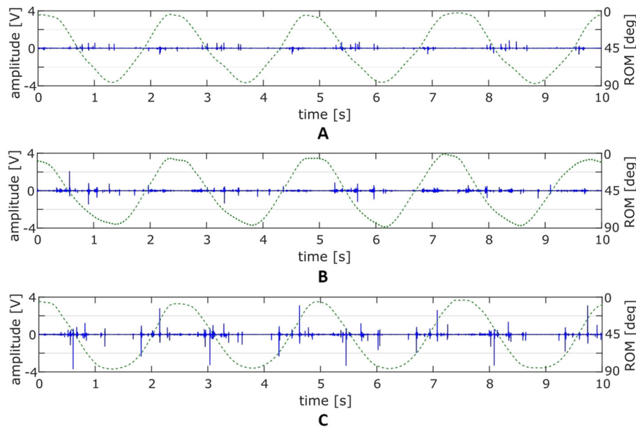
Fig. 3 The course of representative vibroarthrographic signals for conditions (a) with no load (b) with 10 kg load (c) with 20 kg load
