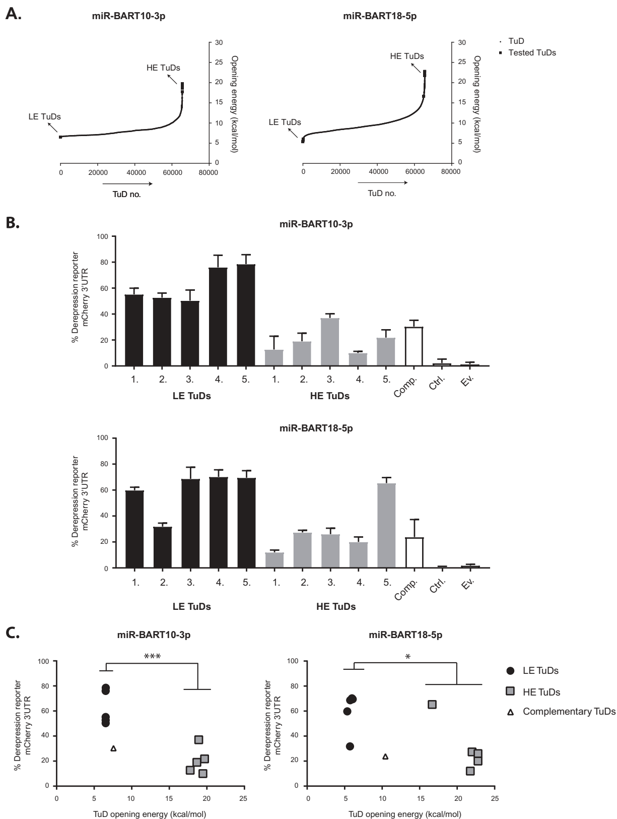
Figure 4. TuD opening energy predicts the inhibitory effect on miRNA functioning.
