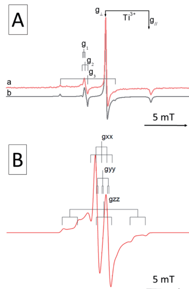
Fig. 6 EPR spectra of N-F doped anatase TiO 2 (A) with the signals of the two independent centers ( \text{NO}^{2-\cdot} and \text{Ti}^{3+} ) and (B) EPR spectrum recorded in N-W co-doped material showing a center containing interacting N and W dopants. This part of the figure is adapted with permission from ref. 57.
