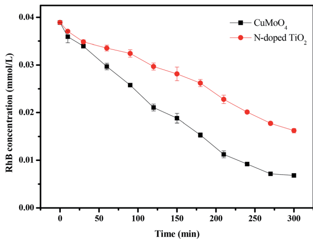
Fig. 18 The photocatalytic degradation of rhodamine B under visible light irradiation with \text{CuMoO}_4 and N-doped \text{TiO}_2 as the photocatalyst, respectively.
