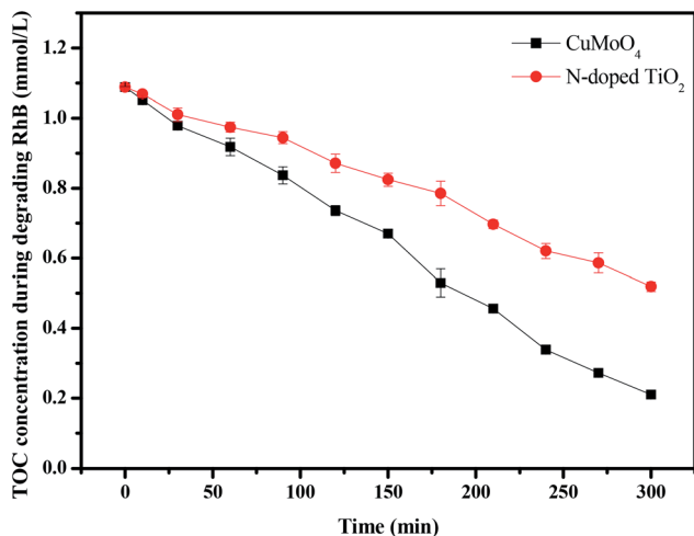
Fig. 19 TOC plots during the photocatalytic degradation of rhodamine B under visible light irradiation with \text{CuMoO}_4 and N-doped \text{TiO}_2 as the photocatalyst, respectively.
