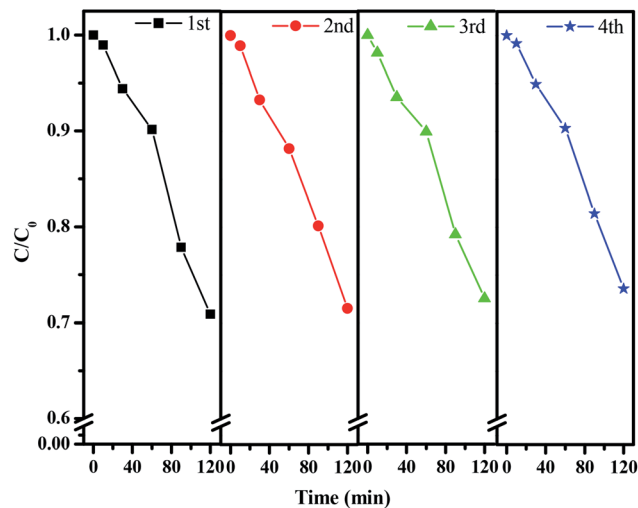
Fig. 20 Repeated photocatalytic degradation tests of rhodamine B with \text{CuMoO}_4 as the photocatalyst.
