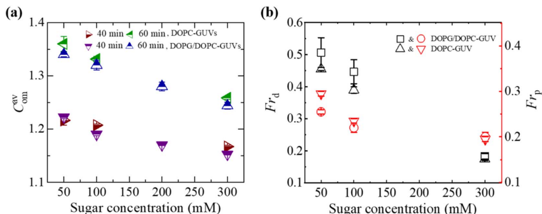
Fig. 4 Sugar concentration dependent C_{om}^{av} , Fr_d , and Fr_p in DOPG/DOPC (40/60)-GUVs and DOPC-GUVs interacted with 3.33 \mu\text{g}/\text{mL} MNPs. (a) Sugar concentration dependent C_{om}^{av} at 40 and 60 min. (b) Sugar concentration dependent Fr_d and Fr_p at 40 min. The figures have been adapted from ref. 52 with permission from PLOS, copyright 2022.
