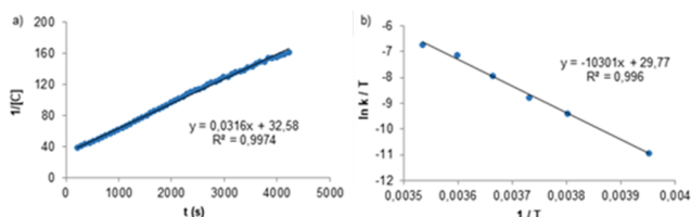
Figure 7. (a) Second-order kinetic representation for the consumption of 4a at -5 °C in CD 2 Cl 2 . (b) Eyring plot for ethane formation from gem-digold methyl [Au 2 (μ-CH 3 )(PMe 2 Ar Xyl12 ) 2 ][NTf 2 ] (4a).
