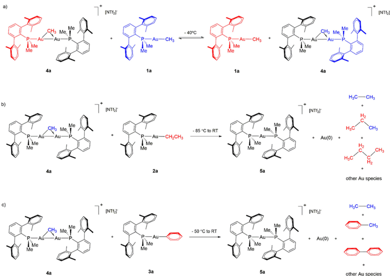
Scheme 6. (a) Dynamic Me/Me Exchange Equilibrium between [Au 2 (μ-CH 3 )(PMe 2 Ar Xyl12 ) 2 ][NTf 2 ] (4a) and Au(CH 3 )(PMe 2 Ar Xyl12 ) (1a) Species at -40 °C; (b) C–C Coupling and Product Distribution in the Reaction between Au(C 2 H 5 )(PMe 2 Ar Xyl12 ) (2a) and [Au 2 (μ-CH 3 )(PMe 2 Ar Xyl12 ) 2 ][NTf 2 ] (4a); and (c) C–C Coupling and Product Distribution in the Reaction between Au(C 6 H 5 )(PMe 2 Ar Xyl12 ) (3a) and [Au 2 (μ-CH 3 )(PMe 2 Ar Xyl12 ) 2 ][NTf 2 ] (4a)
