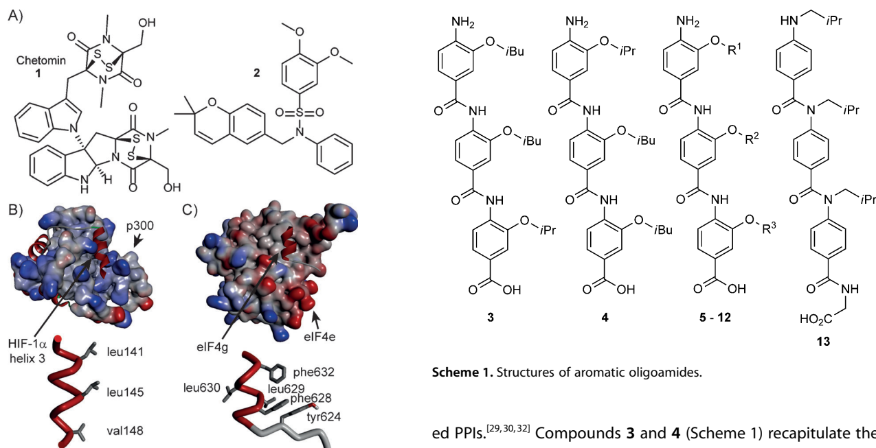
Figure 1. A) Structures of previously reported inhibitors: natural product chetomin ( 1 ) [13] and synthetic compound 2 reported by Van Meir. [14] B) NMR structure (PDB ID: 1L8C) [5] of p300 in complex with the C-terminal transactivation domain of HIF-1 \alpha (top) and excised C-terminal helix of HIF-1 \alpha showing key side chains (bottom). C) X-ray crystal structure (PDB ID: 2W97) [15] of the eIF4E-eIF4G complex (top) and the excised helix of eIF4G showing key side chains (bottom).
