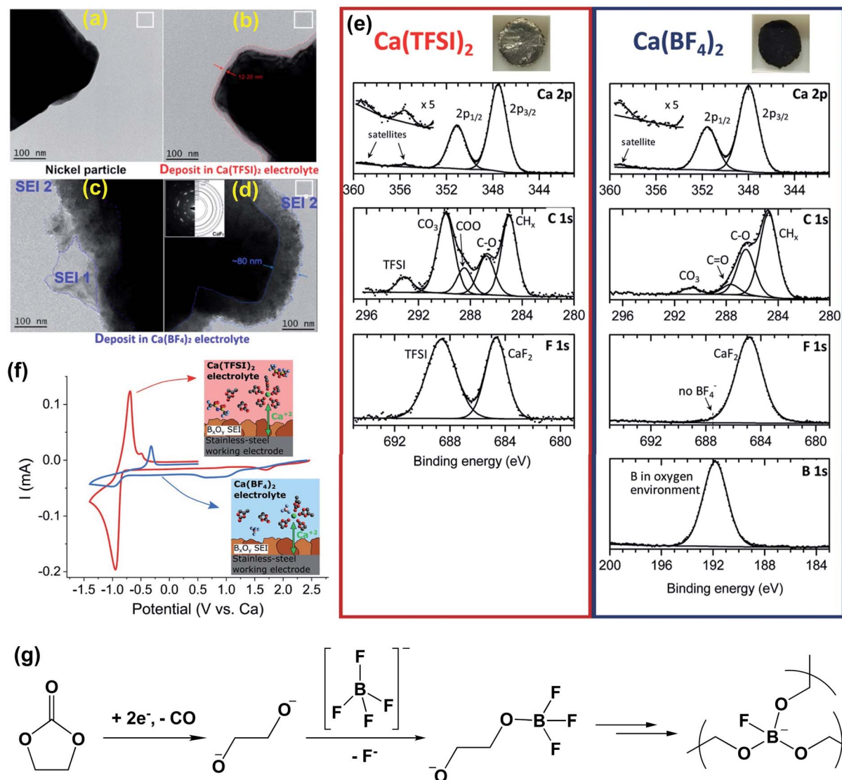
Fig. 5 Surface characterization of the Ca anode in \text{Ca}(\text{BF}_4)_2 -EC/PC (50 : 50 wt%) and \text{Ca}(\text{TFSI})_2 -EC/PC electrolytes. (a–d) Bright field TEM images of Ni particles (working electrode) before and after the formation of a surface layer. (e) XPS spectra of the passivation layers formed on a calcium disk in the \text{Ca}(\text{TFSI})_2 electrolyte (left panel) and the \text{Ca}(\text{BF}_4)_2 electrolyte (right panel), respectively; insets show the appearance of each calcium disk after negative polarization for 48 hours. (f) Cyclic voltammograms ( 0.1 \text{ mV s}^{-1} ) of pre-passivated stainless-steel electrodes (covered with borate films) using either \text{Ca}(\text{TFSI})_2 (red curve) or \text{Ca}(\text{BF}_4)_2 (blue curve) electrolytes. Insets show the proposed cation solvation structures in each electrolyte. (g) Proposed decomposition mechanism for the \text{Ca}(\text{BF}_4)_2 -EC/PC electrolyte to form a proposed \text{BO}_3 polymer. Adapted with permission from ref. 25. Copyright 2020 Royal Society of Chemistry.
