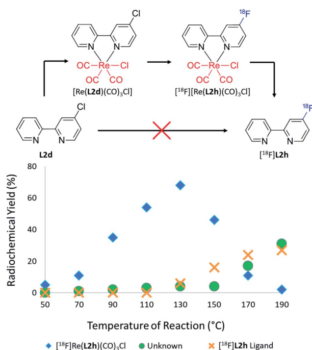
Fig. 4 RCYs of [\text{Re}(\text{L2h})(\text{CO})_3\text{Cl}] (blue diamonds), [\text{Re}(\text{L2h})\text{Ligand}] (orange crosses) and an unknown by-product (green circles) plotted as a function of the reaction temperature for the [\text{Re}(\text{CO})_3(\text{L2d})\text{Cl}] complex. [\text{Re}(\text{L2h})\text{Ligand}] was unable to be synthesised from \text{L2d} unless mediated by rhenium(i) complexation as per the above scheme.
