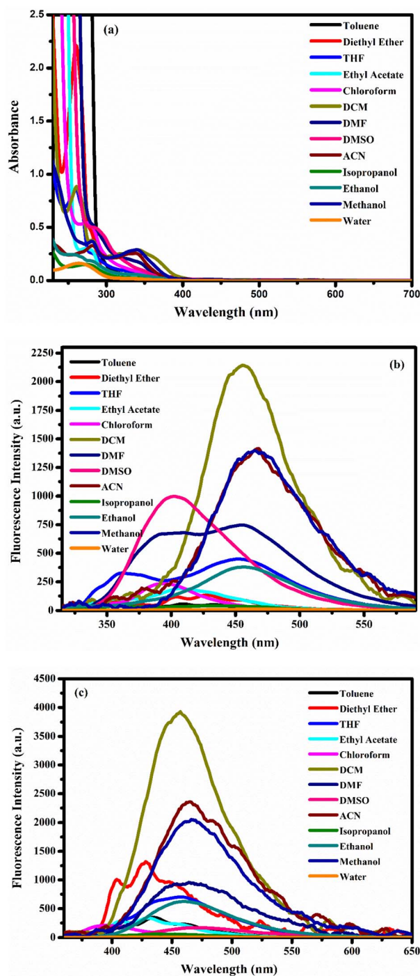
Fig. 2 (a) The UV-vis absorption and (b) \lambda_{exc} = 300 nm fluorescence spectra and (c) \lambda_{exc} = 350 nm fluorescence spectra of compound C 18 (10 \mu M) in different solvents.
