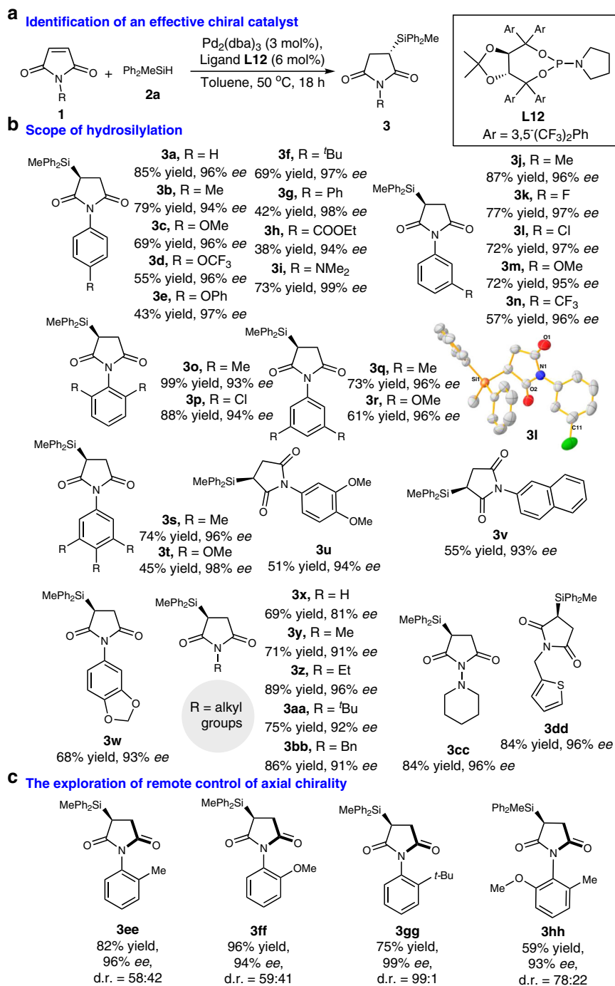
Fig. 2 Enantioselective palladium-catalysed hydrosilylation of maleimides. a The determination of chiral palladium catalyst after screening of a variety of chiral ligands and reaction parameters, and that corresponding to L12 is optimal. b The catalytic asymmetric hydrosilylation of maleimides is broadly applicable, affording silyl products with excellent enantioselectivities (up to 99% ee). Products containing 5-heterocycle and unsubstituted imide can be accessed. c The effect of bulky groups at the ortho -position of N -arylmaleimides on enantioselective Si-C coupling hydrosilylation with respect to the remote control of axial chirality.
