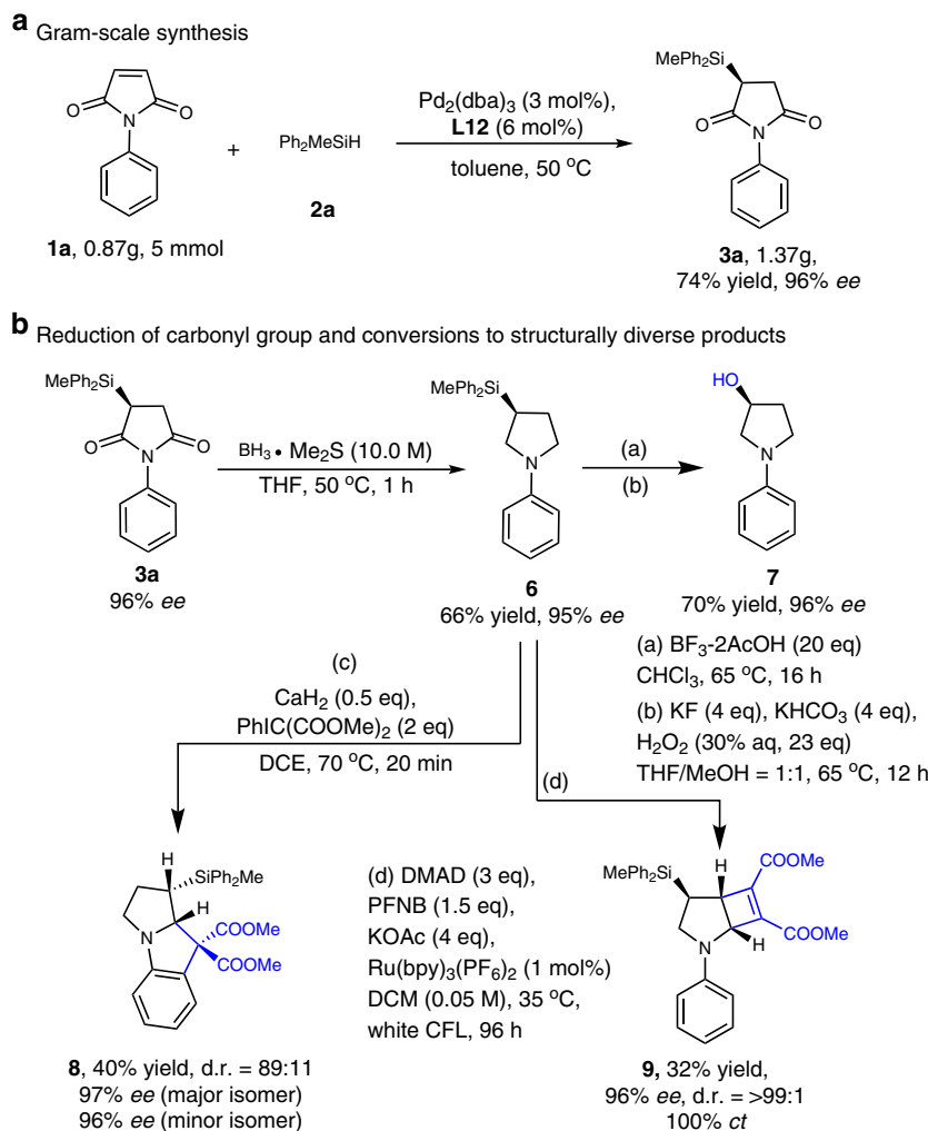
Fig. 4 Gram-scale synthesis and functionalisation and demonstration of utility. a Gram-scale reaction. Compared with the small-scale reaction, using substrates 1a and 2a in a gram-scale reaction produced the desired product 3a with the same level of enantiomeric excess (ee) and yield. b The silyl succinimides can be readily reduced to the stable silylpyrrolidine that could be transferred into structurally diverse and chiral N -heterocycles without racemisation. DMAD dimethyl acetylenedicarboxylate, PFNB pentafluoronitrobenzene, CFL compact fluorescent light, ct the value of chirality transfer.
