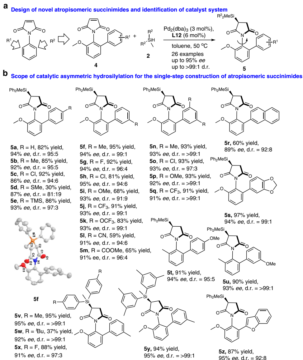
Fig. 3 Remote control of axial chirality of C-N bond by hydrosilylation. a The design of C-N bond rotatable atropisomers by introduction of two different substituents on the ortho -position of N -arylmaleimides to stabilise axial chirality. b The catalytic asymmetric hydrosilylation is broadly applicable in the construction of atropisomeric N -arylmaleimides with good chemo-, diastereo-, and enantioselectivity and in up to 97% yield. Products containing sp 3 central chirality and axial chirality can be accessed in the single step of Si-C coupling hydrosilylation.
