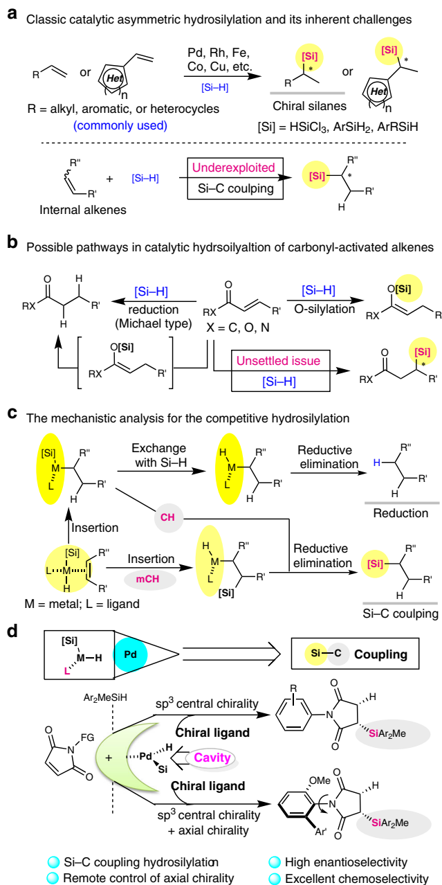
Fig. 1 Chemo- and stereo-selective issues with hydrosilylation. a Catalytic asymmetric hydrosilylation of terminal alkenes mediated by transition-metal catalysts. b Traditional methods for hydrosilylation of EWG-activated alkenes led to reduction and O -silylation. c Two classic pathways for transition-metal-catalysed hydrosilylation of alkenes, and its mechanistic analysis should encourage greater adoption of Si–C coupling methods for the hydrosilylation of internal alkenes. d The catalytic desymmetric hydrosilylation of N -arylmaleimides for remote control of axial chirality. CH is Chalk–Harrod mechanism, and mCH is modified Chalk–Harrod mechanism.
