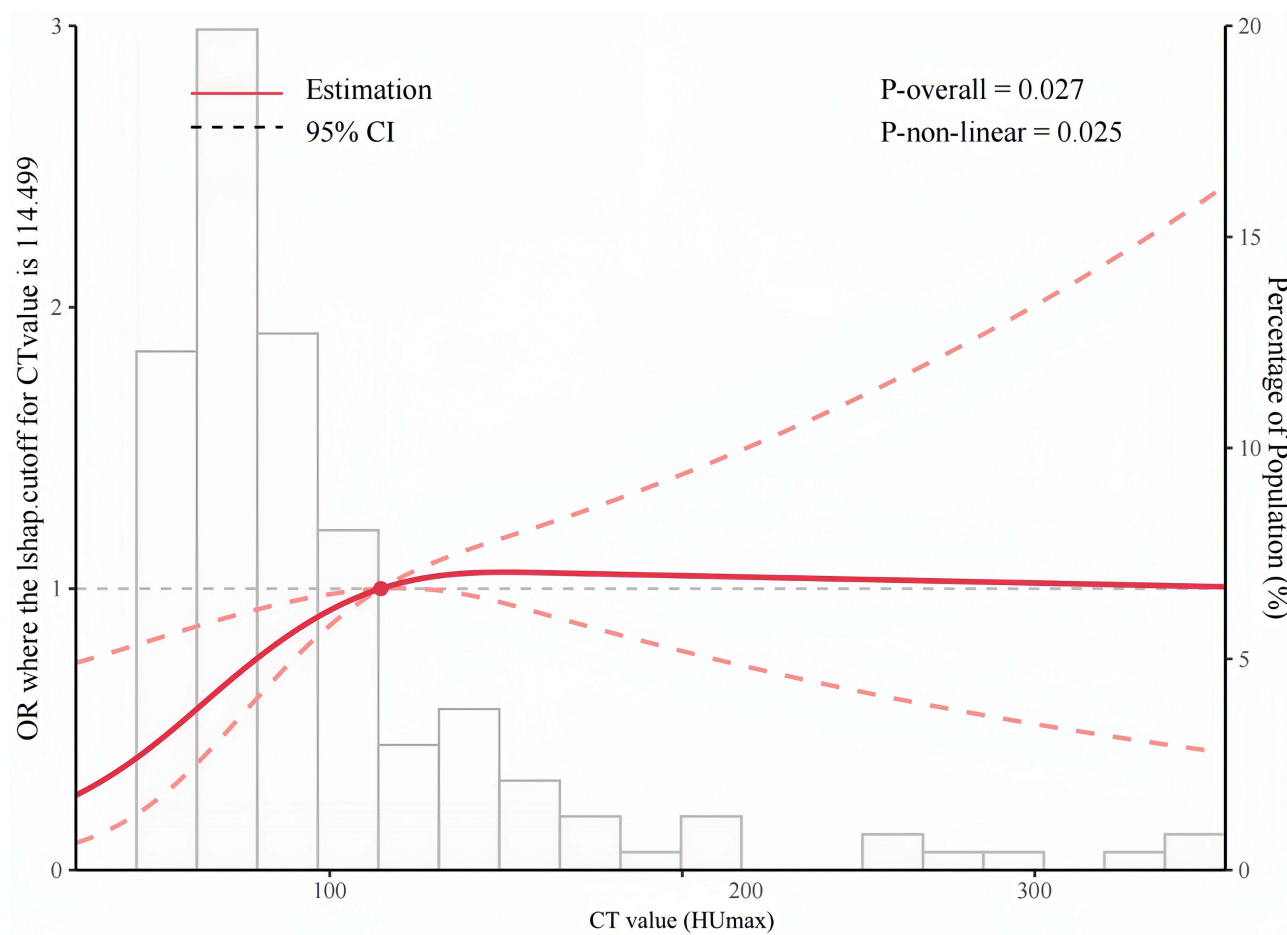
Figure 4 Restricted cubic spline (RCS) for the associations between maximum CT value and SAP. The lines represent odds ratios (ORs, solid lines) and 95% confidence intervals (CIs, long dashed lines) after multivariable adjustment for all confounding factors based on the RCS models. The reference values (OR = 1) were set at the 50th percentiles, and the knots were set at the 10th, 50th, and 90th percentiles of the maximum CT value. The histograms represent the distribution of CT value in our study, excluding values outside the 5th and 95th percentiles.
