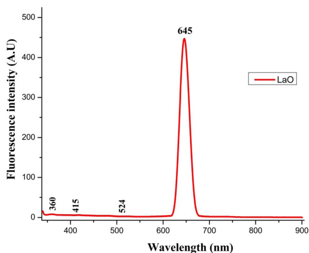
Fig. 6 Fluorescence spectrum of La 2 O 3 NPs.
