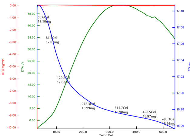
Fig. 5 TGA of La 2 O 3 NPs.
