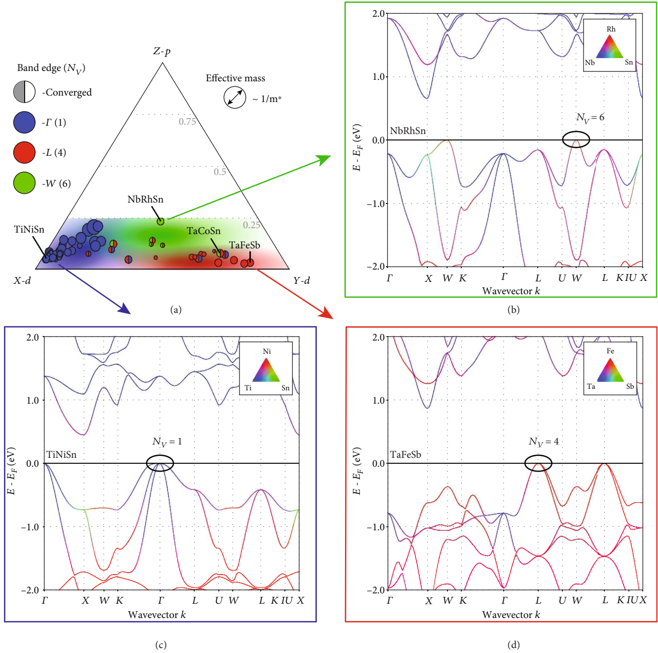
FIGURE 2: (a) The valence band edges of half-Heusler electronic structures are primarily composed of d orbitals from the X - and Y -sites, and secondarily, p orbitals from the Z -site. The relative contributions of these basis orbitals describe the type of carrier pockets observed in this structure family. (b) Electronic structures with higher concentrations of Z - p orbitals at the band edge have carrier pockets at the W -point with high degeneracy. (c) Phases with valence band edges dominated by X - d states have carrier pockets at the \Gamma -point, and (d) band edges dominated by Y - d states have carrier pockets at the L -point.
