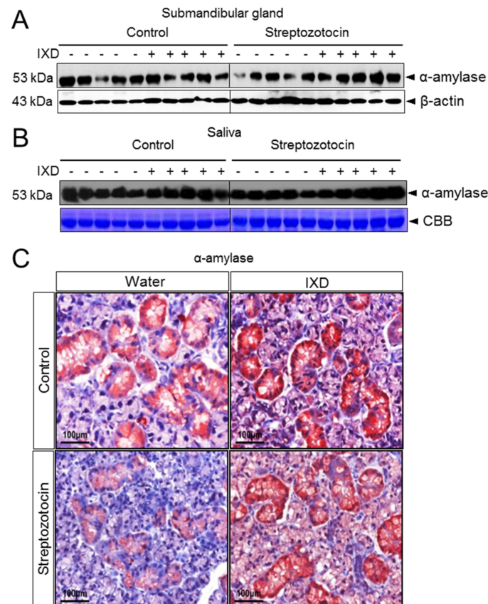
Figure 4. Expression of \alpha -amylase in the submandibular gland and saliva. (A) Amylase expression in submandibular gland tissue lysates; (B) amylase expression in saliva; (C) paraffin-embedded submandibular gland tissues were sectioned at 5 \mu m thickness, and immunostaining was performed using an amylase antibody. Brownish red colours indicate immunolocalization of \alpha -amylase in submandibular gland cells. Magnification: 40 \times ; Scale bar: 100 \mu m.
