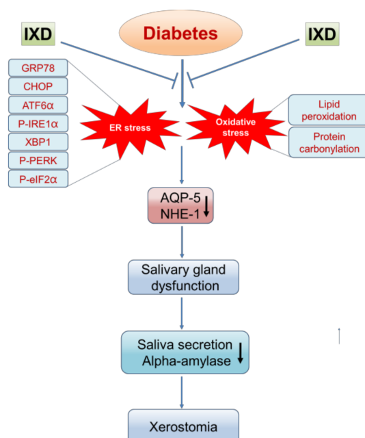
Figure 8. The proposed mechanism of an IXD extract against diabetes-induced xerostomia. The schematic diagram shows diabetes-associated ER stress and oxidative stress, subsequently, altering the protein expression of AQP5 and NHE1 in the submandibular gland. This may cause salivary gland dysfunction with reduction in salivary secretion leading to xerostomia. This graphic shows that IXD extract increases salivary secretion through the regulation of ER stress and prevents from xerostomia.
