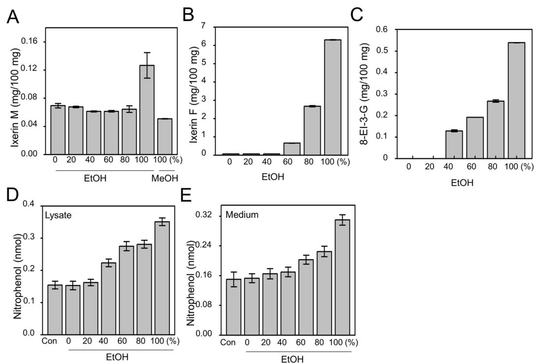
Figure 1. The effect of the different grades of ethanol on extraction of IXD. Purified compounds, (A) Ixerin M; (B) Ixerin F; (C) epiisolidiol-3- \beta -D-glucopyranoside (8-EI-3-G) in the IXD extract found by extraction with different grades of ethanol and 100% methanol; (D,E) effect of different grades of ethanol on extraction of IXD and measurement of amylase secretion in HSG cells exposed to high glucose concentrations; (D) amylase secretion measurement using cell lysates; (E) amylase secretion measurement using cell cultured medium.
