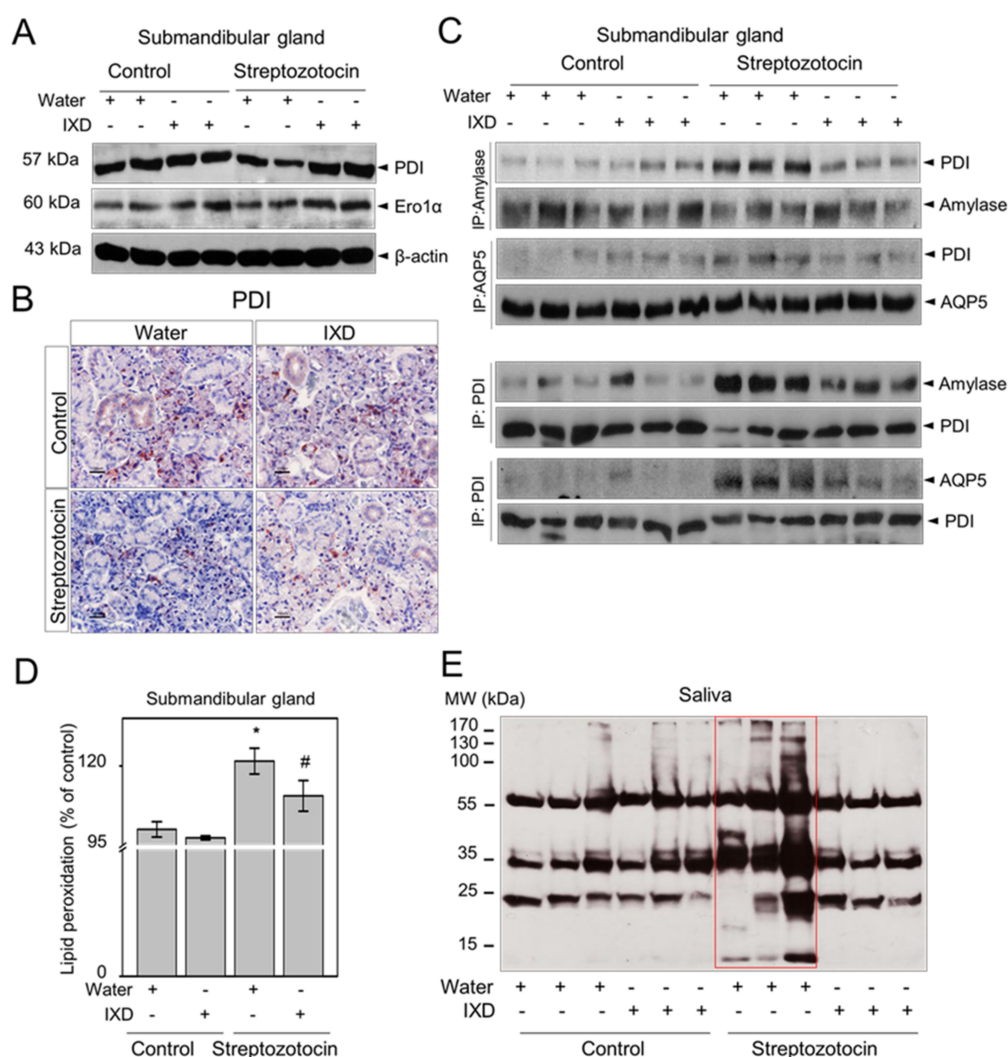
Figure 7. The IXD extract regulates ER folding environment. (A) Western blot analysis showing the expression of PDI and ERO1 \alpha in submandibular gland lysates; (B) immunostaining of PDI in the submandibular gland. Magnification 40 \times ; Scale bar: 100 \mu m; (C) submandibular gland lysates were immunoprecipitated with anti-amylase or AQP5 antibody and immunoblotted with the anti-PDI (upper), anti-amylase or anti-AQP5 antibody (lower); (D) TBARS assay was performed to measure lipid peroxidation level in vehicle or IXD-treated submandibular gland homogenates. Values are expressed as percentage of control, ( n = 10 per group, p < 0.05 ). * indicates significant differences compared to vehicle-treated control rats and # indicates significant differences compared to STZ-induced diabetic control rats; E: Detection of salivary carbonyls using Western blotting. The molecular weight (MW) is indicated in kDa. Red rectangular box shows the high protein carbonylation pattern in the saliva of STZ-induced diabetic rats.
