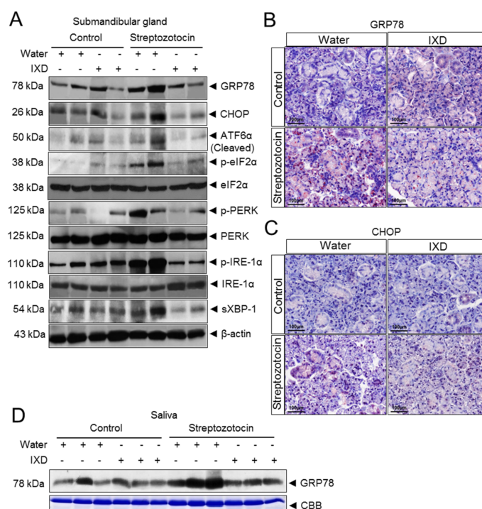
Figure 6. The IXD extract regulates the ER stress response in submandibular gland of diabetic rats. (A) Western blot analysis was performed to demonstrate the ER stress response using GRP78, CHOP, ATF6 \alpha , p-eIF2 \alpha , total eIF2 \alpha , p-PERK, total PERK, p-IRE1 \alpha , total IRE1 \alpha , and sXBP-1 antibodies. An equal concentration of protein (30 \mu g) was loaded in each lane of the gels. Beta-actin was used as a loading control. The molecular weight of each protein is indicated in kDa; (B) immunostaining of GRP78; (C) immunostaining of CHOP in the submandibular gland. Magnification: 40 \times ; Scale bar: 100 \mu m; (D) expression of secreted GRP78 in saliva in the indicated groups. Coomassie Brilliant Blue (CBB) staining was performed as a control for equal protein loading.
