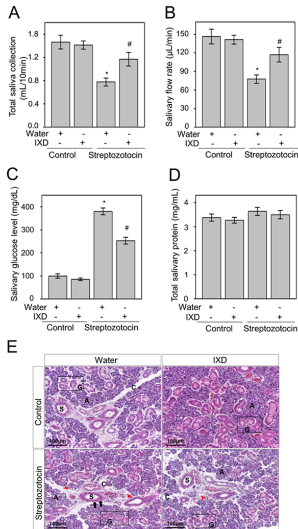
Figure 3. The effects of the IXD extract on salivary parameters. (A) Total salivary volume (mL) collected at 10 min after pilocarpine injection; (B) the total salivary flow rate was measured in \mu\text{L}/\text{min} ; (C) measurement of glucose concentration in saliva; (D) measurement of total protein concentration in saliva (mg/mL). Values are represented as mean \pm SEM ( n = 10 per group, p < 0.05 ). * indicates significant differences compared to vehicle-treated control rats and # indicates significant differences compared to STZ-induced diabetic rats; (E) haematoxylin and eosin staining showing the morphological appearance of the submandibular glands of control and diabetic rats. Red arrowheads show variable degrees of vacuolization of the connective tissue stroma. Black arrows show slightly dilated and pyknotic nuclei in striated ducts. Characters showing in pictures such as A, C, S and G denotes for acinar cells, connective tissue stroma, striated ducts and granular convoluted tubules respectively. Magnification: 20\times ; Scale bar: 100\ \mu\text{m} .
