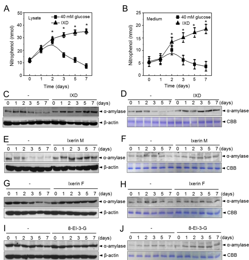
Figure 2. The IXD extract increases amylase synthesis and secretion in human salivary gland cells exposed to high glucose levels. (A,B) Amylase activity was measured in cell lysates (A) and cultured medium (B) of HSG cells exposed to high glucose concentrations with or without the IXD extract for 1, 2, 3, 5, and 7 days. Values are represented as mean \pm SEM ( n = 3 , p < 0.05 ). * indicates significant differences with the IXD-untreated cell condition; (C,D) amylase expression in cell lines exposed to high glucose concentrations treated with or without the IXD extract for the indicated time period; (C) amylase protein expression was analysed using cell lysates; (D) amylase protein expression was analysed using cell cultured medium; (E,F) HSG cells were exposed to high glucose concentrations (40 mM) for 1, 2, 3, 5, and 7 days in the presence or absence of Ixerin M, a purified IXD component, and amylase expression was measured in cell lysates (E) and cell medium (F); (G,H) amylase protein expression was analysed in cell lysates or cultured medium in the presence or absence of Ixerin F and (I,J) epiisolidiol-3- \beta -D-glucopyranoside (8-EI-3-G).
