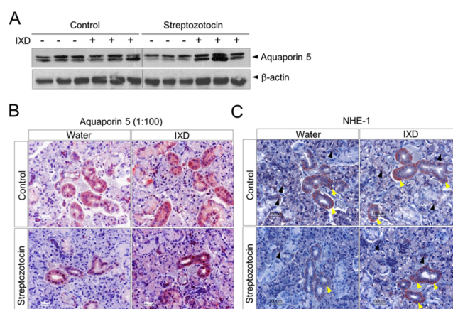
Figure 5. Expression of AQP5 and NHE1 in the submandibular gland. (A) Western blot analysis showing AQP5 protein expression in submandibular gland tissue lysates. The blot identified two bands of AQP5 (27 kDa and 31 kDa) revealing non-glycosylated and glycosylated forms of the AQP5 protein respectively; (B) the expression of AQP5 (1:100) was performed on submandibular gland tissue sections of either water or IXD extract-treated control or diabetic rats. Brownish red colour indicates the positive expression of AQP5. Magnification: 40 \times ; Scale bar: 100 \mu m; (C) immunohistochemical detection of NHE1 in submandibular gland tissue from normal and diabetic rats treated with water or the IXD extract. Yellow arrow heads show the expression of NHE1 in duct cells, whereas black arrow heads indicate acinar expression. Magnification: 40 \times ; Scale bar: 100 \mu m.
