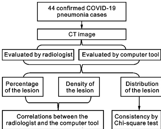
Fig. 1. Study flowchart.
