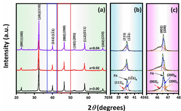
Fig. 1 X-ray diffraction patterns of (1 - x)[0.99\text{BNKT}-0.01\text{BMN}]-x\text{CSO} ceramics: (a) 2\theta = 20^\circ-70^\circ , (b) 2\theta = 38^\circ-42^\circ , and (c) 2\theta = 45^\circ-48^\circ .
