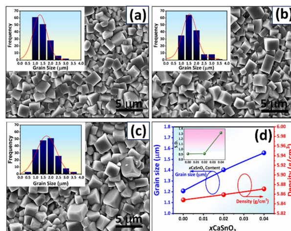
Fig. 3 SEM micrographs of (1 - x)(0.99\text{BNKT}-0.01\text{BMN})-x\text{CSO} sintered ceramics: (a) x = 0.00 , (b) x = 0.02 , (c) x = 0.04 , and (d) grain size with their corresponding density value as a function of CSO content. Insets (a)–(c): grain size distributions of the samples. Inset (d): S.D. vs. CSO content.
