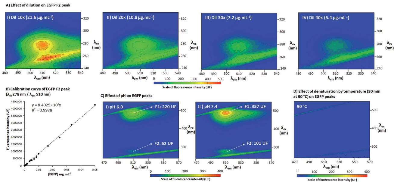
Fig. 3 (A) 3D fluorescence spectra at PB pH 7.4 at 25 °C of different concentrations of EGFP ((A.I) – dil 10×, 21.6 \mu\text{g mL}^{-1} ; (A.II) – dil 20×, 10.8 \mu\text{g mL}^{-1} ; (A.III) – dil 30×, 7.2 \mu\text{g mL}^{-1} ; (A.IV) – dil 40×, 5.4 \mu\text{g mL}^{-1} ), range \lambda_{\text{ex}} 240–330 nm and \lambda_{\text{em}} 480–540 nm, scale of fluorescence intensity 0–500 UF. (B) Calibration curve for EGFP F2 peak ( \lambda_{\text{ex}} 278 nm/ \lambda_{\text{em}} 510 nm), concentration of EGFP [EGFP] ( \text{mg mL}^{-1} ) in the X axis and fluorescence intensity (UF) in the Y axis. (C) 3D fluorescence spectra of EGFP in PB of different pH ((C.I) – pH 6.0 and (C.II) – pH 7.4) and (D) after denaturation by temperature in PB pH 7.4 (30 min at 90 °C), range \lambda_{\text{ex}} 240–550 nm and \lambda_{\text{em}} 470–570 nm, scale of fluorescence intensity (UF) 0–400. 3D fluorescence spectra with the excitation wavelengths in the Y axis ( \lambda_{\text{ex}} ), the emission wavelengths in the X axis ( \lambda_{\text{em}} ) and the scale of fluorescence intensity (UF) according to the color scale from blue to red. F1 (around \lambda_{\text{ex}} 488 nm/ \lambda_{\text{em}} 510 nm) and F2 (around \lambda_{\text{ex}} 296 nm/ \lambda_{\text{em}} 510 nm) are the two fluorescence points with highest intensity. Triplicate measurements with corresponding blank assays for the pH, calibration curve and high temperature experiments, where a representative of the triplicate for the 3D spectra are depicted and the average of the results with respective standard deviations are presented for the calibration curve.
