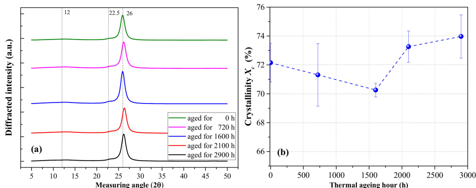
Figure 2. (a) X-ray diffraction (XRD) curves and (b) calculated crystallinity X_c of thermally aged PET films aged at 110 °C.
