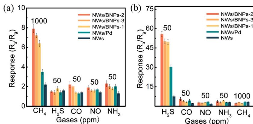
Fig. 11 Selectivity of W_{18}O_{49} NWs/BNPs-2 at (a) 320\text{ }^\circ\text{C} and (b) 100\text{ }^\circ\text{C} to various gases. 68 Reproduced with permission from ref. 68. Copyright 2022, Elsevier.
