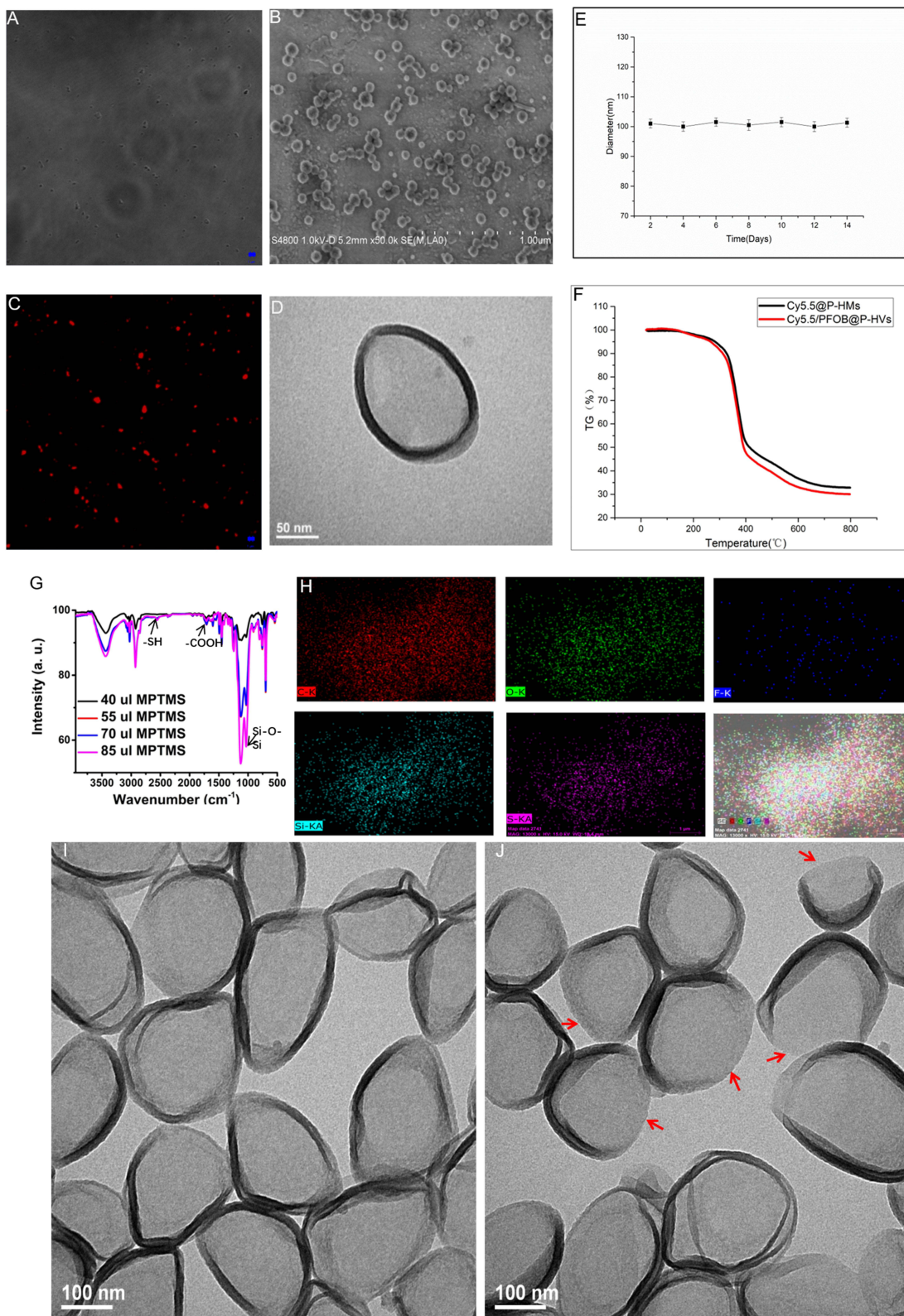
Figure 1 Manifestation of PFOB@P-HVs. (A) Optical microscope. (B) SEM image. (C) Confocal laser scanning microscopy (D) TEM image. (E) Size distribution of PFOB@P-HVs in PBS with time tested by DLS. (F) PFOB encapsulation rate measured by thermogravimetric analysis. (G) FT-IR. (H) EDS element mapping results of PFOB@P-HVs. (I) Nanovesicles morphology before HIFU irradiation. (J) Nanovesicles swollen and ruptured after HIFU stimulation. Red arrowhead: the margin of the ruptured shell.
