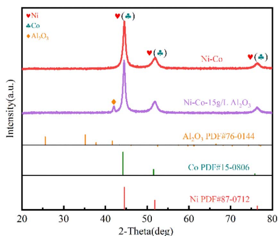
Fig. 4 XRD patterns of the Ni–Co coating and Ni–Co– 15 \text{ g L}^{-1} \text{ Al}_2\text{O}_3 superhydrophobic composite coating.
