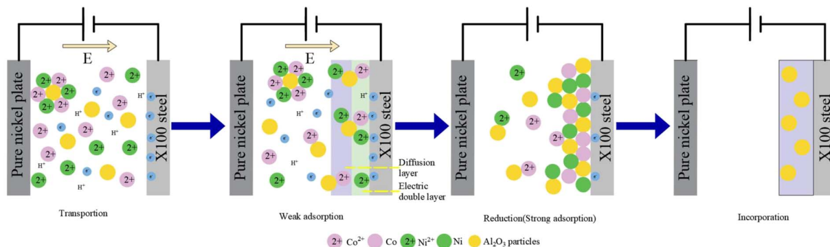
Fig. 3 Electrodeposition mechanism of the Ni–Co– \text{Al}_2\text{O}_3 composite coating.
