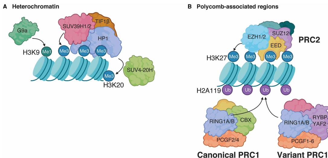
Figure 2. Heterochromatin and Polycomb-associated regions are distinct forms of epigenetically silenced chromatin. (A) Heterochromatin is marked by H3K9me3 deposited by the suppressor of variegation (SUV) 39-homologue enzymes (SUV39H1 and SUV39H2). These enzymes preferentially bind already monomethylated substrate (H3K9me1). H3K9me3 is recognised by heterochromatin protein 1 (HP1) which self-oligomerizes causing compaction of chromatin and rendering it inaccessible to the transcriptional machinery. HP1 in turn recruits SUV4-20H enzymes which deposit another histone mark of heterochromatin H3K20me3. (B) Polycomb-associated regions are particularly involved in cell-type-specific silencing of developmentally regulated genes and are marked by H3K27me3 deposited by the Polycomb repressive complex (PRC) 2 and H2A119ub1 deposited by the PRC1 complex. Polycomb-associated regions block transcription initiation but can remain accessible to the binding of transcription factors, unlike heterochromatin.
