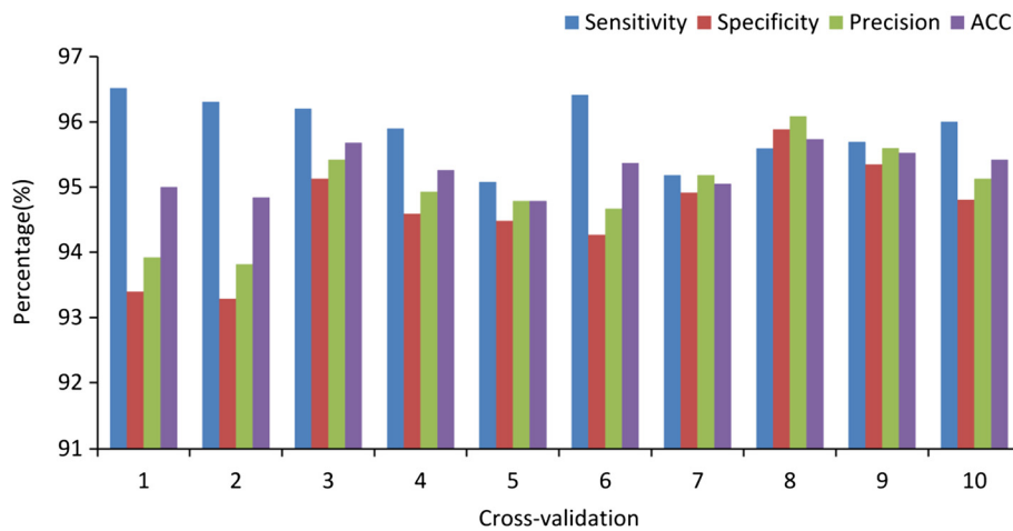
Figure 2 10-cross-validation results.
