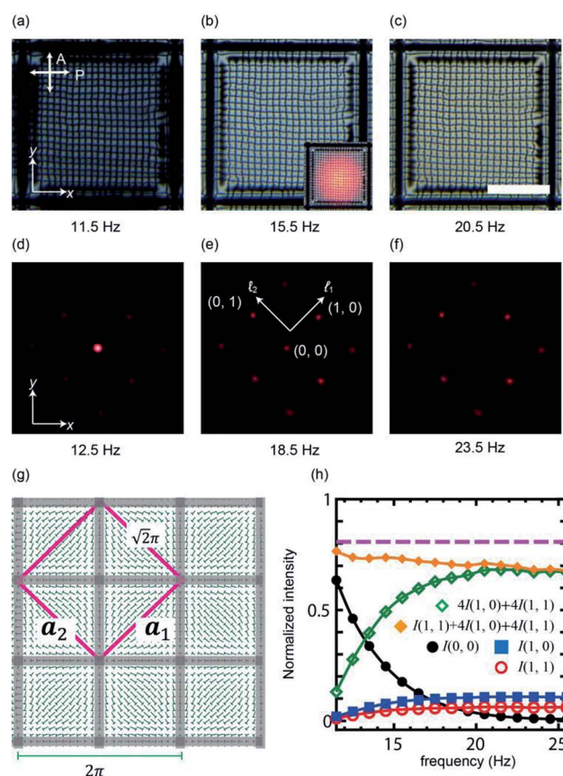
Fig. 2 (a)–(c) The micrographic images for the grid-like texture under cross-polarized condition. Scale bar, 500 \mu\text{m} . The inset of (b) is a micrograph of a grid-like texture irradiated with a laser beam. (d)–(f) Diffraction patterns obtained by a laser beam irradiation. The incident beam is circularly polarized. The amplitude of the applied voltage is 25 V. (d) 12.5 Hz, (e) 18.5 Hz, (f) 23.5 Hz. (g) A schematic illustration of the director field of the grid-like texture. The square is the unit cell for the light diffraction. Here, we set the lattice constant as \sqrt{2}\pi without loss of generality. (h) The intensity for each spot as a function of frequency. The intensity is normalized with the incident beam. The dashed line is the total power of the light transmitted through the cell. The power meter is placed right behind the cell.
