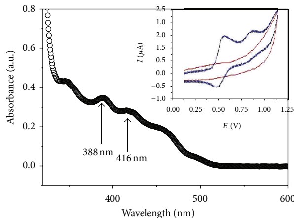
FIGURE 1: Absorption spectra of (tpbi) 2 Ir(acac) material. The inset was cyclic voltammetry curve of the iridium dye.
