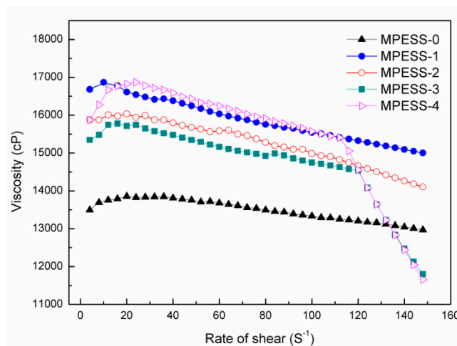
Figure 2. Shear viscosities of the PES/SPES/DMAc/PEG200 casting solutions.
