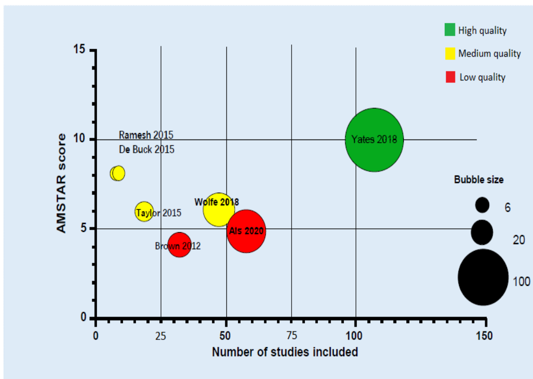
Fig. 4: Evidence mapping
