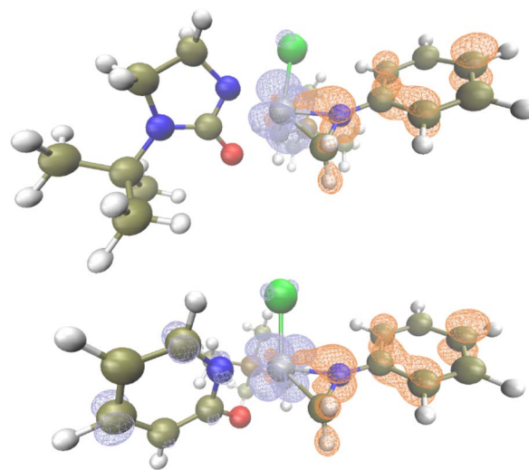
Fig. 1 Excitation analysis of TaL1 (top) and TaL2 in toluene, and electrons (blue) and holes (orange) after excitation (opt: M06L-D3/Def2SVP, TD: M06L-D3/Def2TZVPP, isovalue = 0.05).
