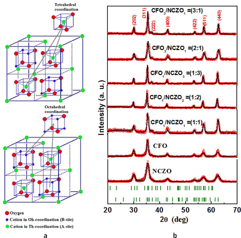
Fig. 1 Features of the crystal structure of the CFO x /NCZO y composites. (a) Crystal structure of the spinel-like ferrite with SG: Fd\bar{3}m . (b) XRD patterns of the CFO x /NCZO y composites.
