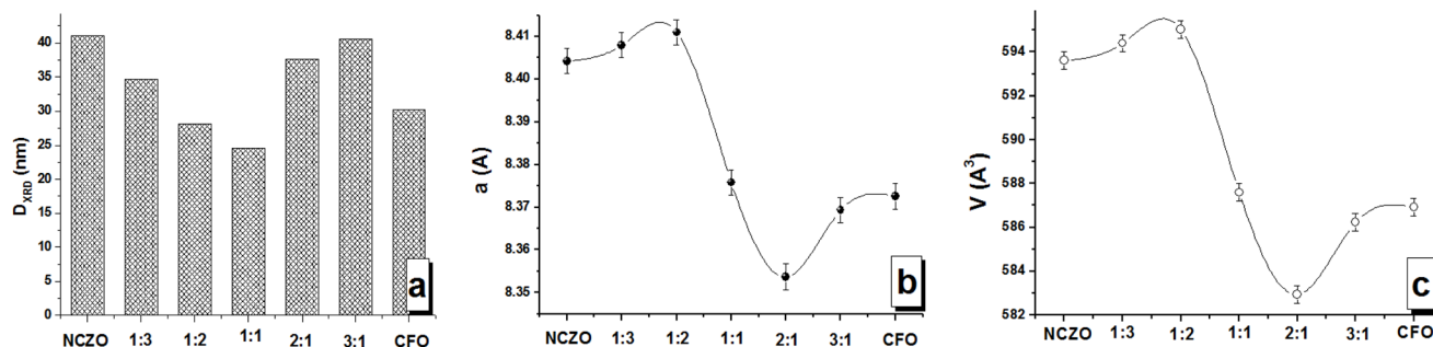
Fig. 2 Main structural parameters of the CFO x /NCZO y composites from XRD data analysis. (a) Average size of crystallite. (b) Lattice parameter a . (c) Volume of the unit cell V .
