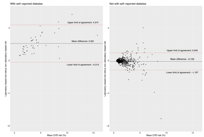
Figure 5 Bland-Altman plots showing agreement between laboratory-based and non-laboratory-based risk scores according to self-reported diabetes status.
