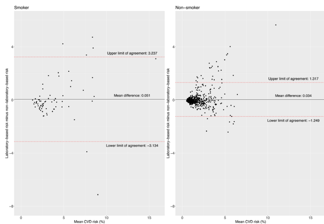
Figure 4 Bland-Altman plots showing agreement between laboratory-based and non-laboratory-based risk scores according to smoking status. CVD, cardiovascular disease.
