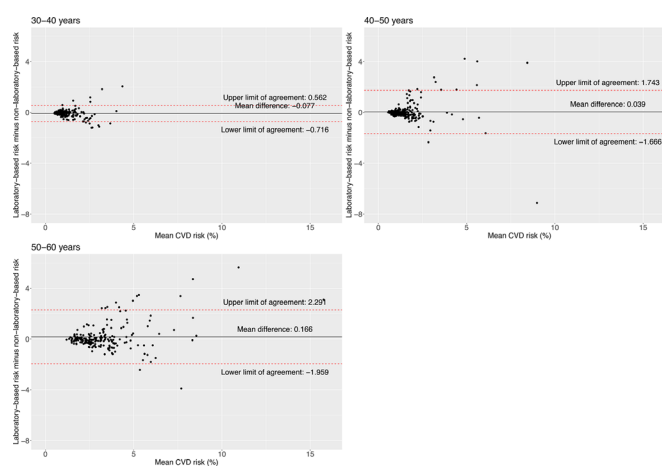
Figure 2 Bland-Altman plots showing agreement between laboratory-based and non-laboratory-based risk scores according to age groups.
