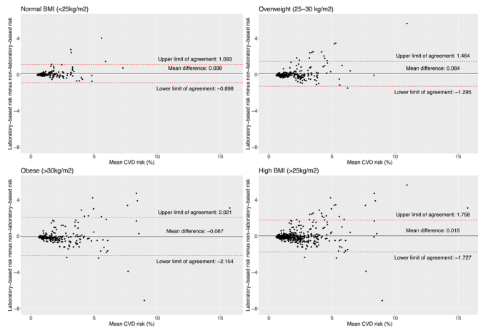
Figure 3 Bland-Altman plots showing agreement between laboratory-based and non-laboratory-based risk scores according to body mass index (BMI) categories.
