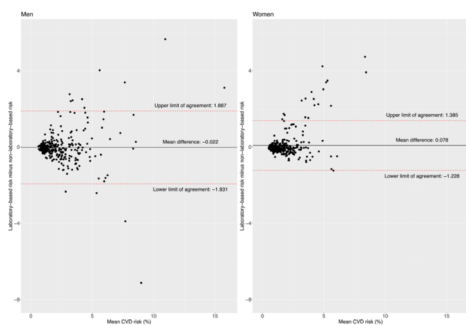
Figure 1 Bland-Altman plots showing agreement between laboratory-based and non-laboratory-based risk scores according to sex.
