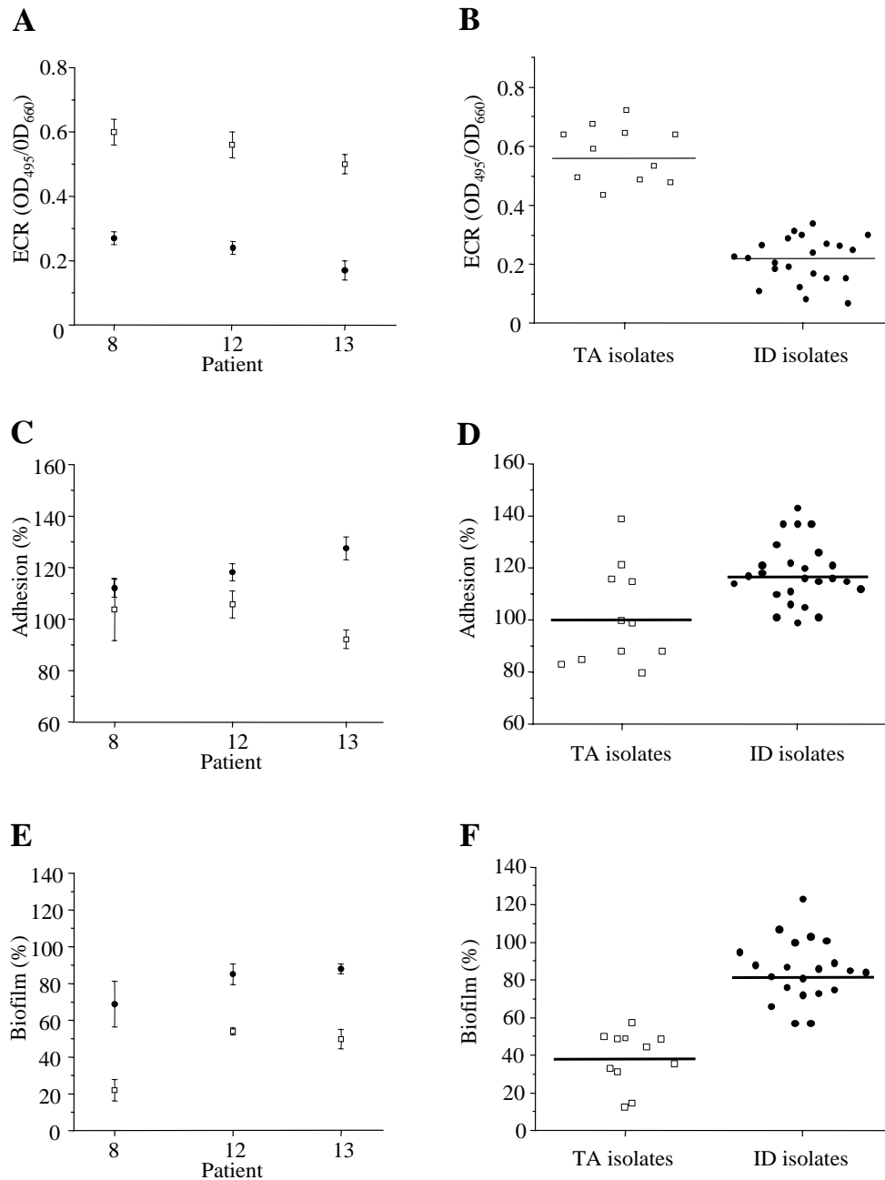
Figure 2 Quorum-sensing dependent phenotypes of P. aeruginosa isolates from tracheal aspirates and intubation devices. Elastase production (A and B), adhesion capacity (C and D) and biofilm formation (E and F) by P. aeruginosa isolates recovered from tracheal aspirates (open squares, TA isolates) and intubation devices (plain circles, ID isolates). Elastolytic activities were determined by ECR assays and expressed as the OD measured at 495 nm per unit of OD 660 nm. The adhesion capacities and biofilm formation were expressed as the percentage relative to the level obtained with the wild-type P. aeruginosa strain PT5. (A, C and E) Results individualized for each patient (8, 12 and 13), error bars correspond to the standard errors of the means. (B, D and F) Mean values and variances for 11 tracheal aspirate isolates and 25 isolates recovered from the intubation devices. For each individual isolate the determinations were performed twice in triplicates.
