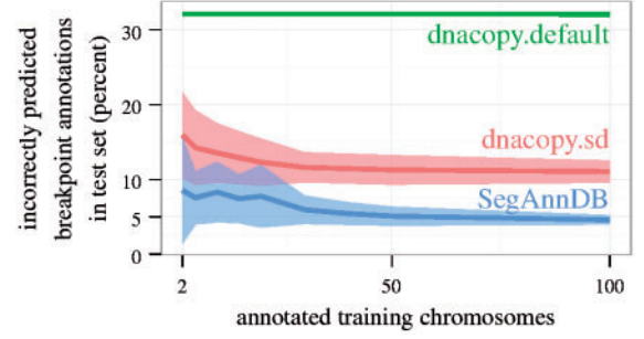
Fig. 4. Cross-validation was used to estimate breakpoint detection error in the neuroblastoma.U830.bac dataset. It is clear that the supervised methods (dnacopy.sd, SegAnnDB) adapt to the training set, and provide better breakpoint detection on test data. Note that dnacopy.sd sometimes had lower test error than SegAnnDB in the other datasets we examined (Supplementary Fig. S5)
