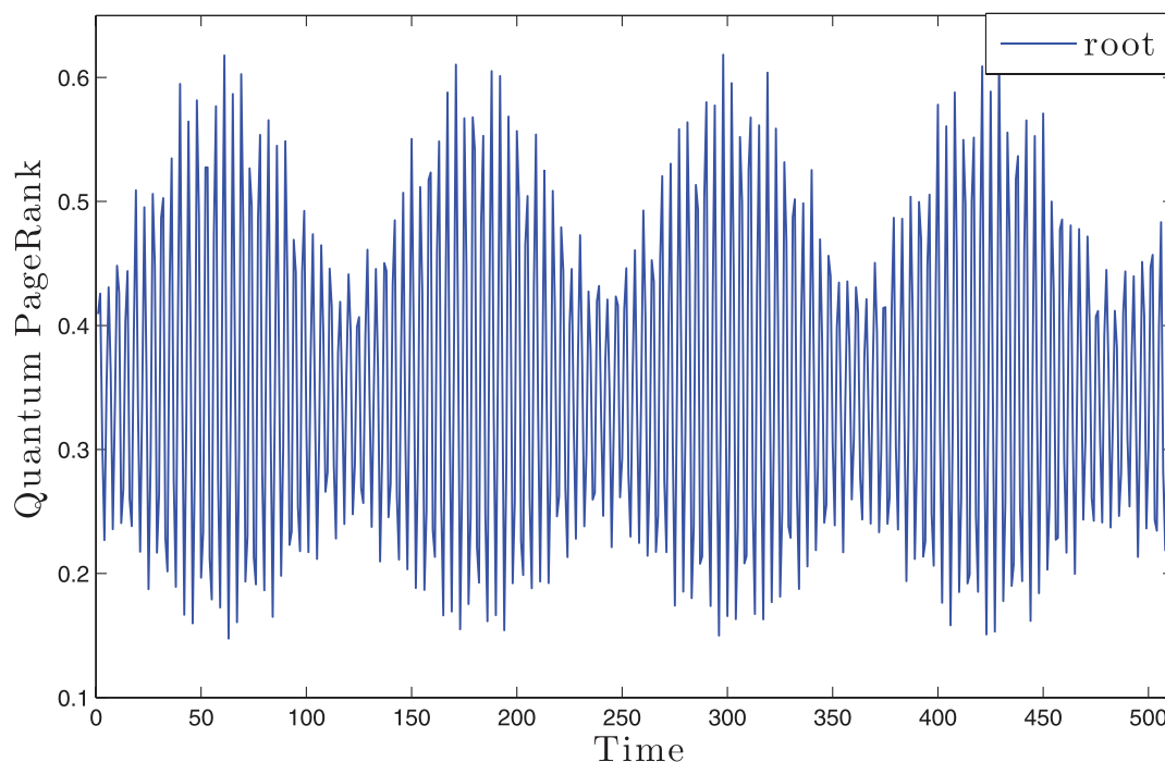
Figure 9 | The evolution of the instantaneous Quantum PageRank I_q with time for the root page (home page) in the case of a directed binary tree in Fig. 7.
